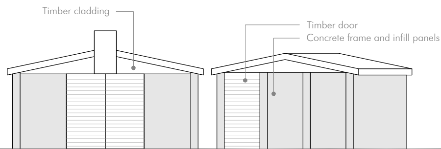
Existing South Elevation - Units 1 & 2
