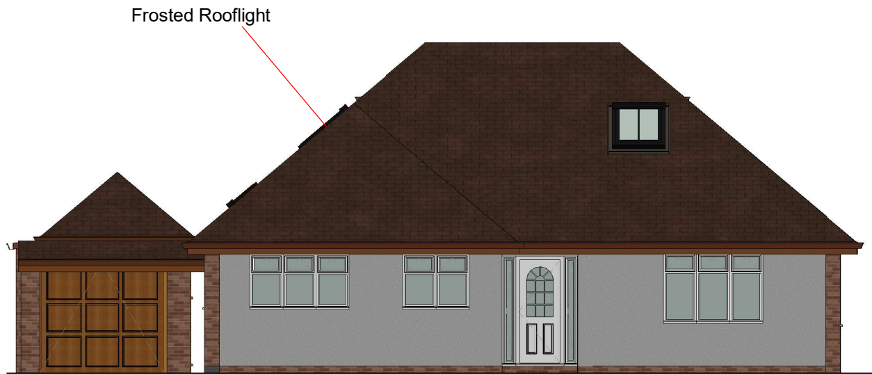
1 North Elevation 1 : 100
