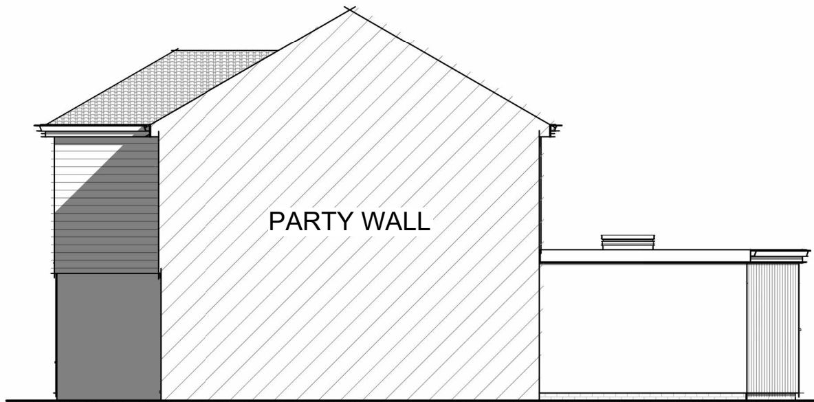
6 Proposed Side (East) 1 : 100
