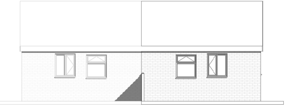
Proposed Elevation-Rear
