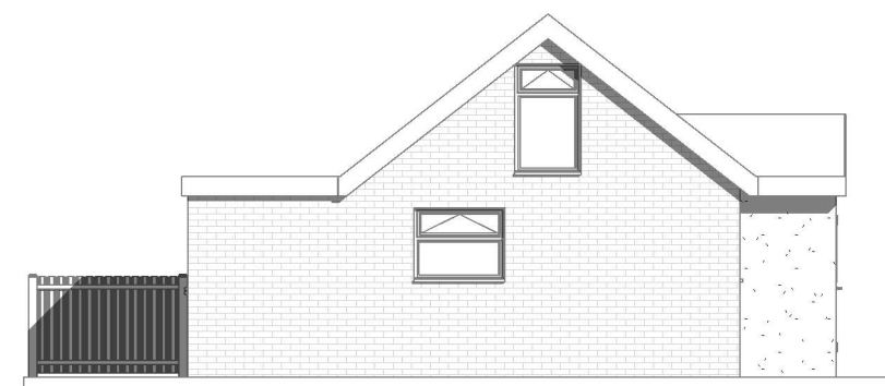
Proposed Elevation-Left side
