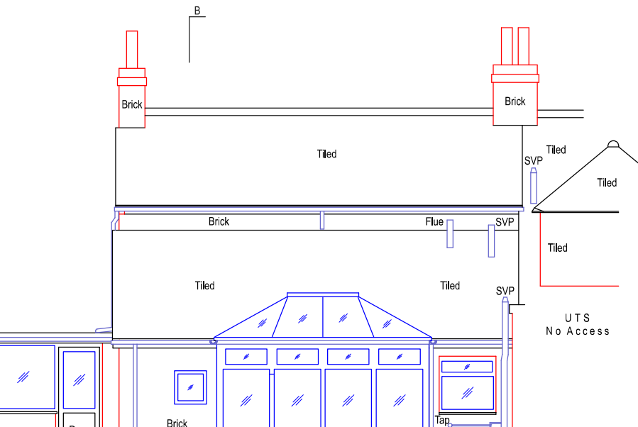
3 REAR ELEVATION 3 (NORTH) Scale: 1:100
