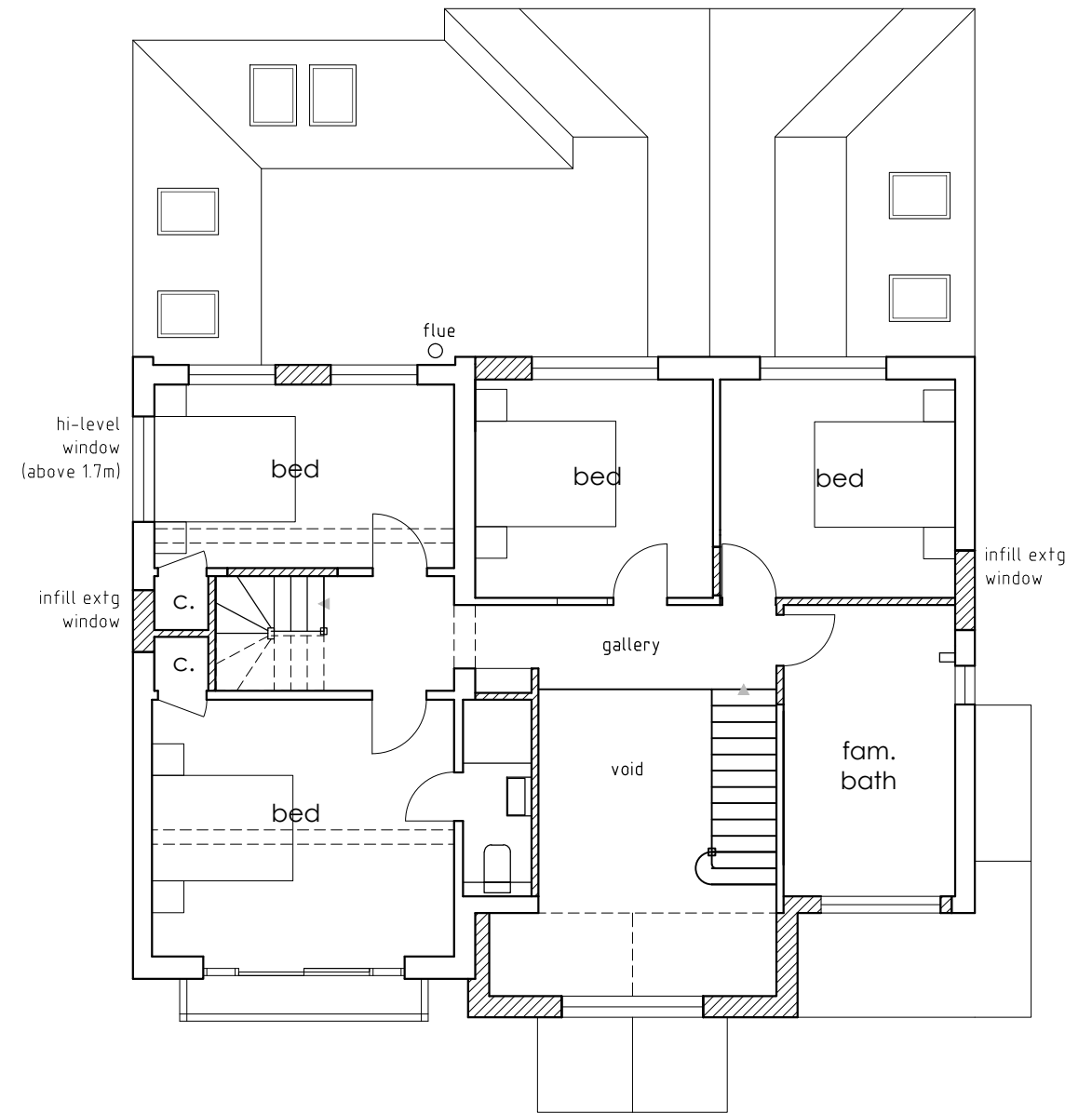
FIRST: PROPOSED 1:100
