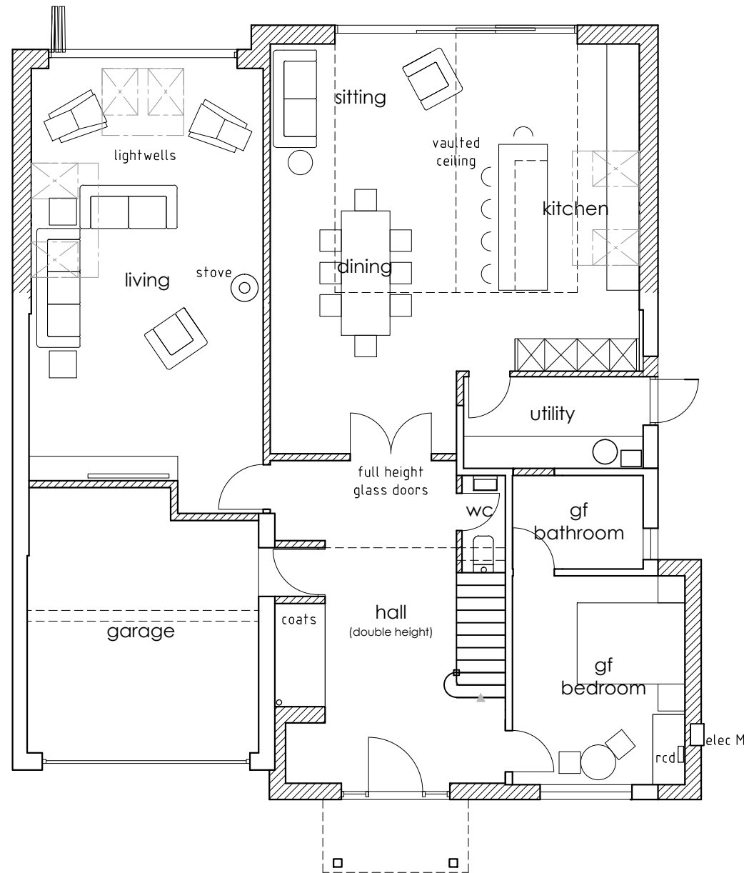
GROUND: PROPOSED 1:100
