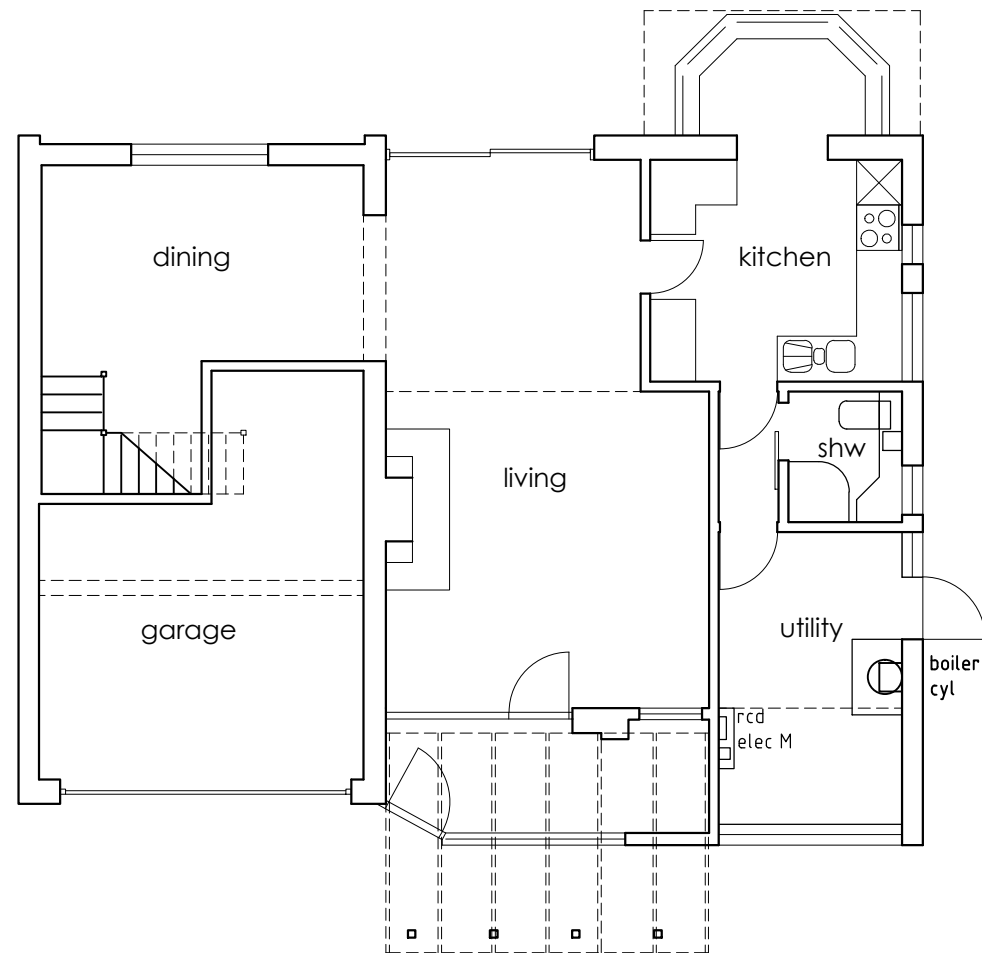
GROUND: EXISTING 1:100
