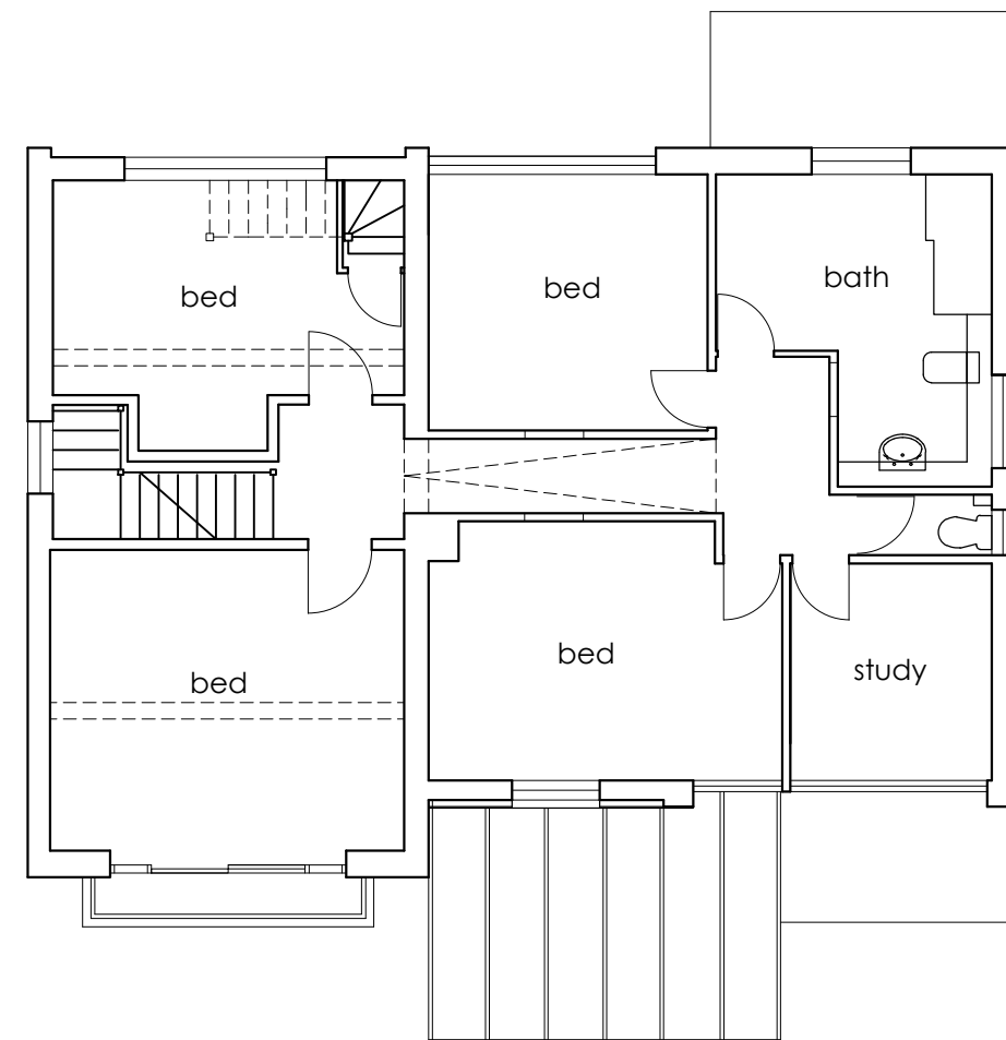
FIRST: EXISTING 1:100
