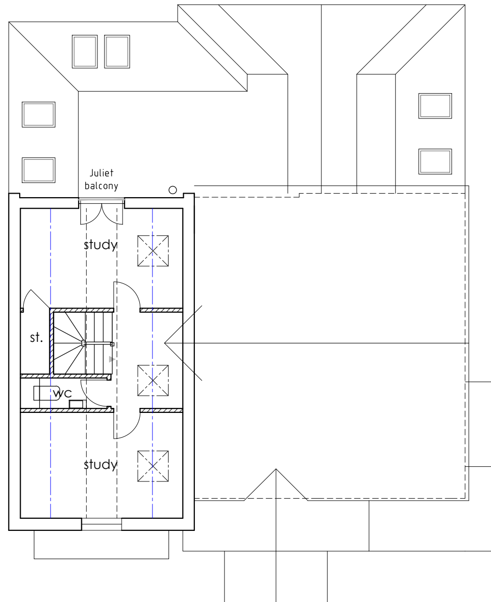
SECOND: PROPOSED 1:100
