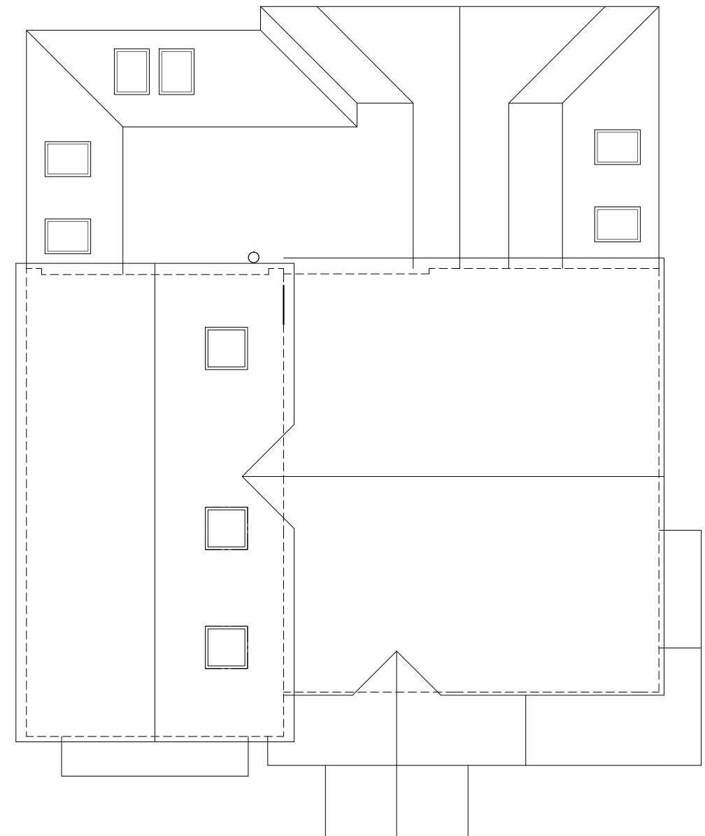
ROOF: PROPOSED 1:100
