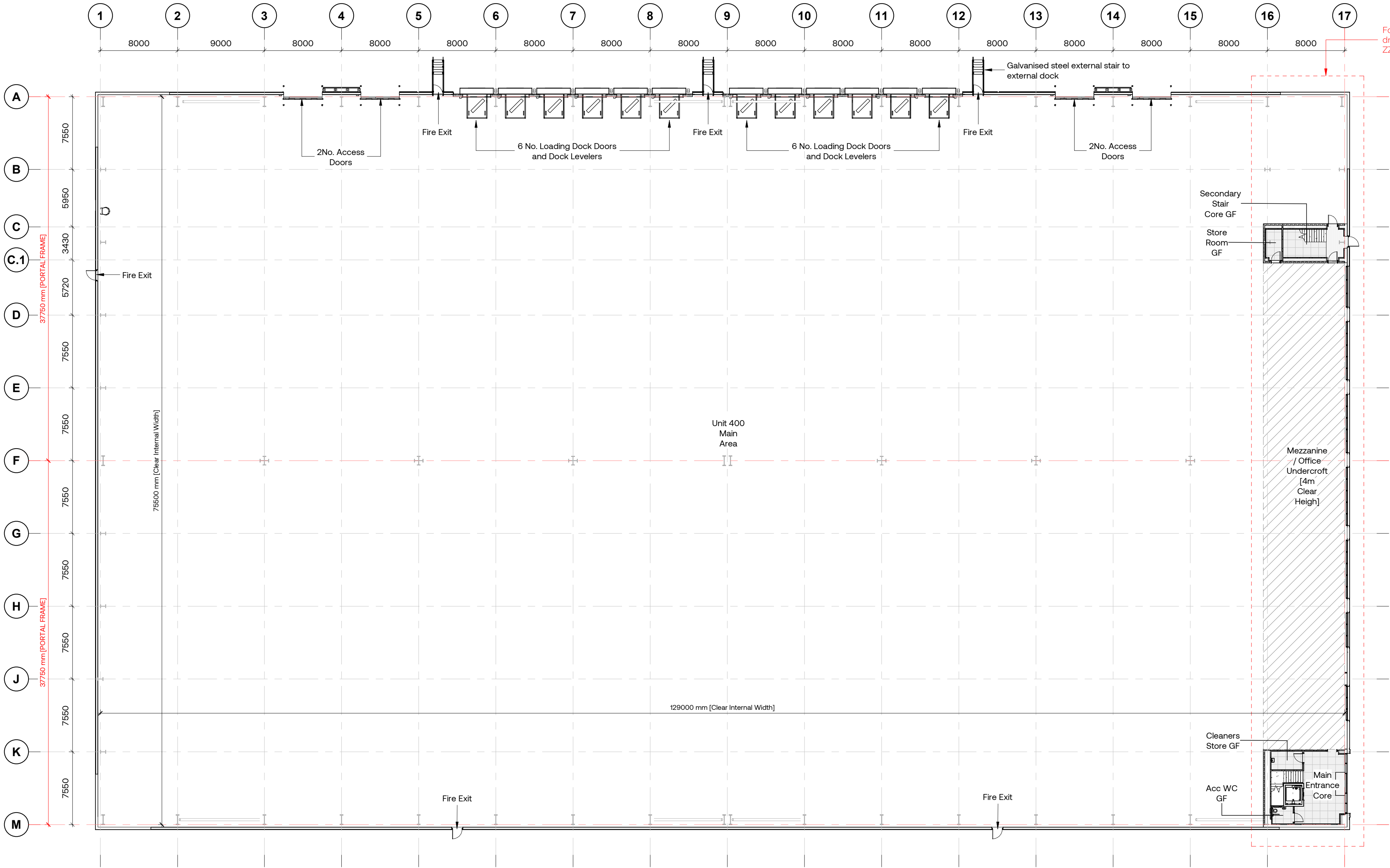
Ground Floor Plan 1:250
