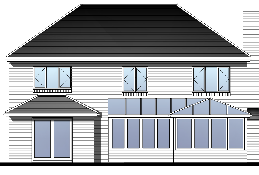
Proposed Rear Elevation (E) 1:100
