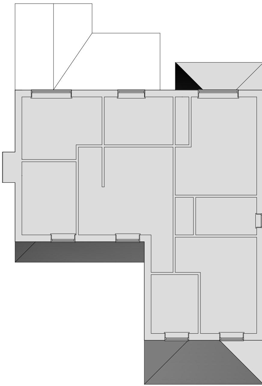
Existing First Floor (Unchanged) 1:100
