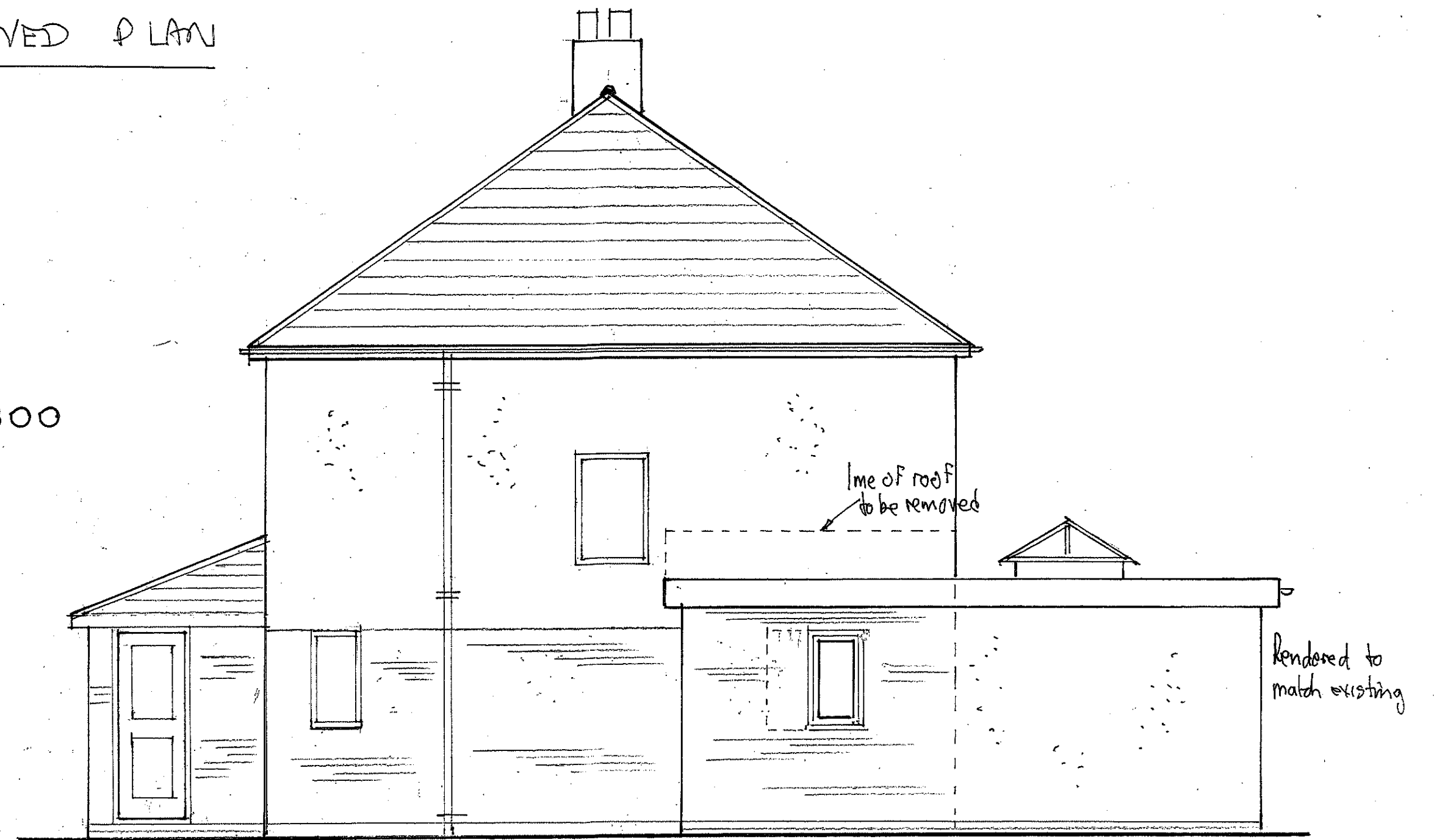
EAST SIDE
