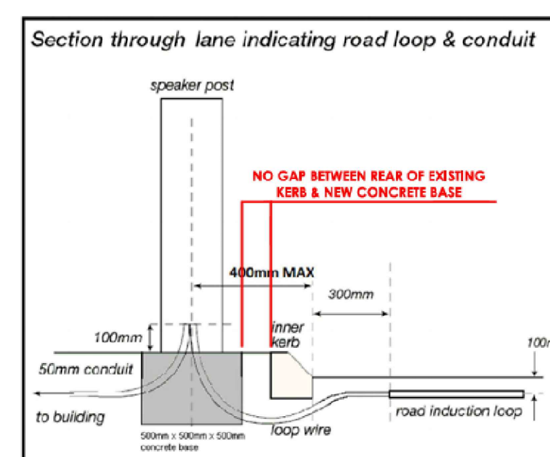
standard Quail Digital timing loop & speaker post setting out details
