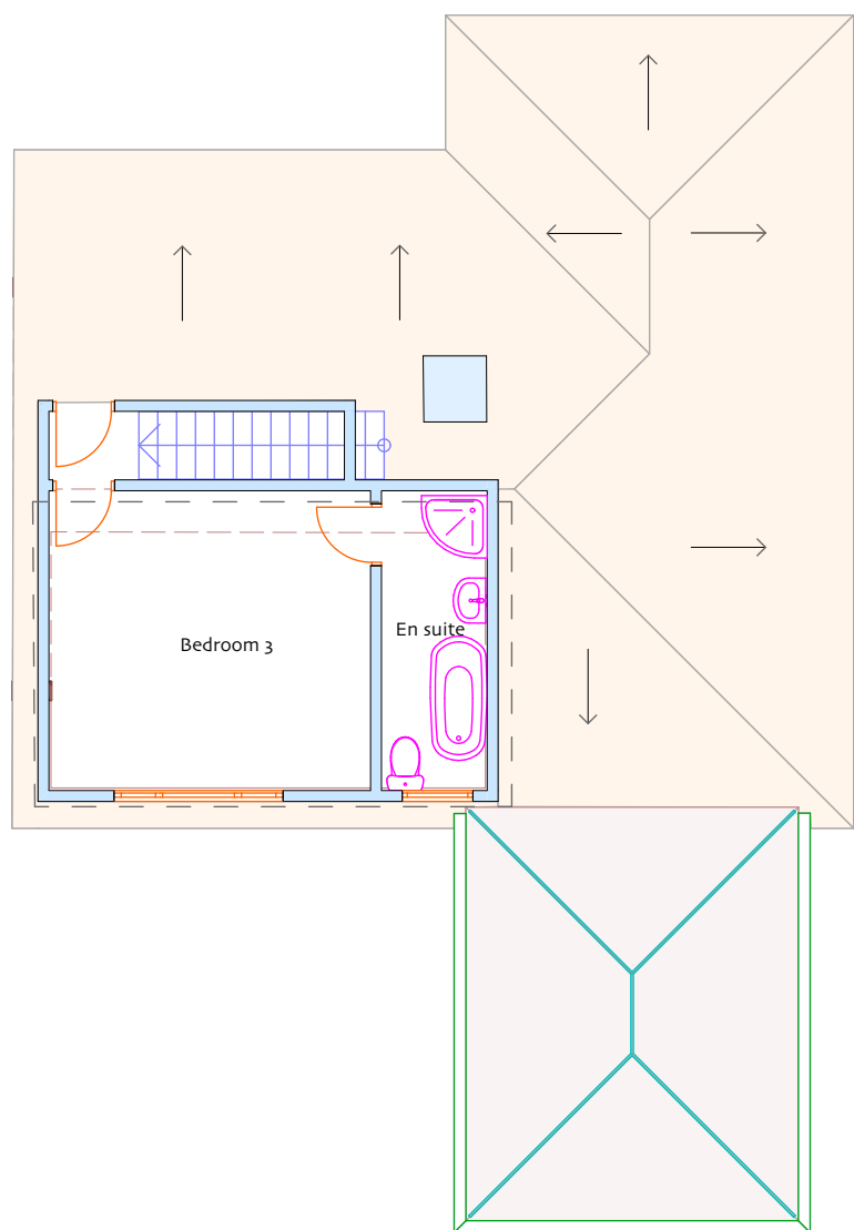
9 - First Floor Existing 1:100
