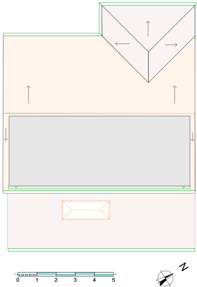
1 Proposed Roof Plans - Roofs at 2 Different Levels - 1:100
