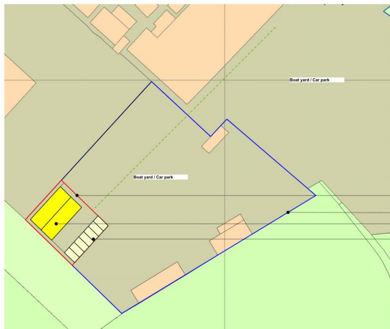
1. Proposed Block plan Scale 1 - 500 @A3
