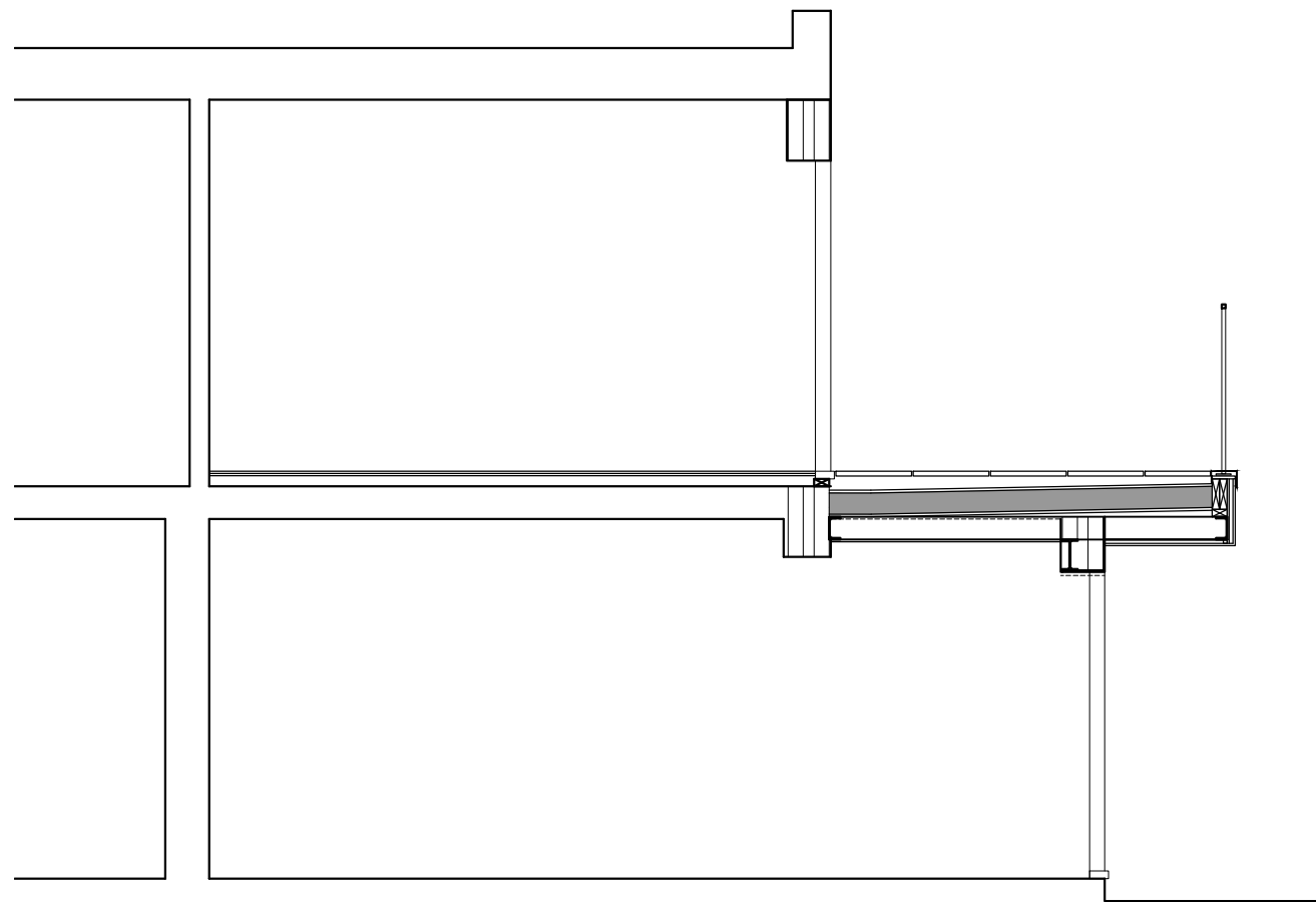
SECTION THRU BALCONY 1:50
