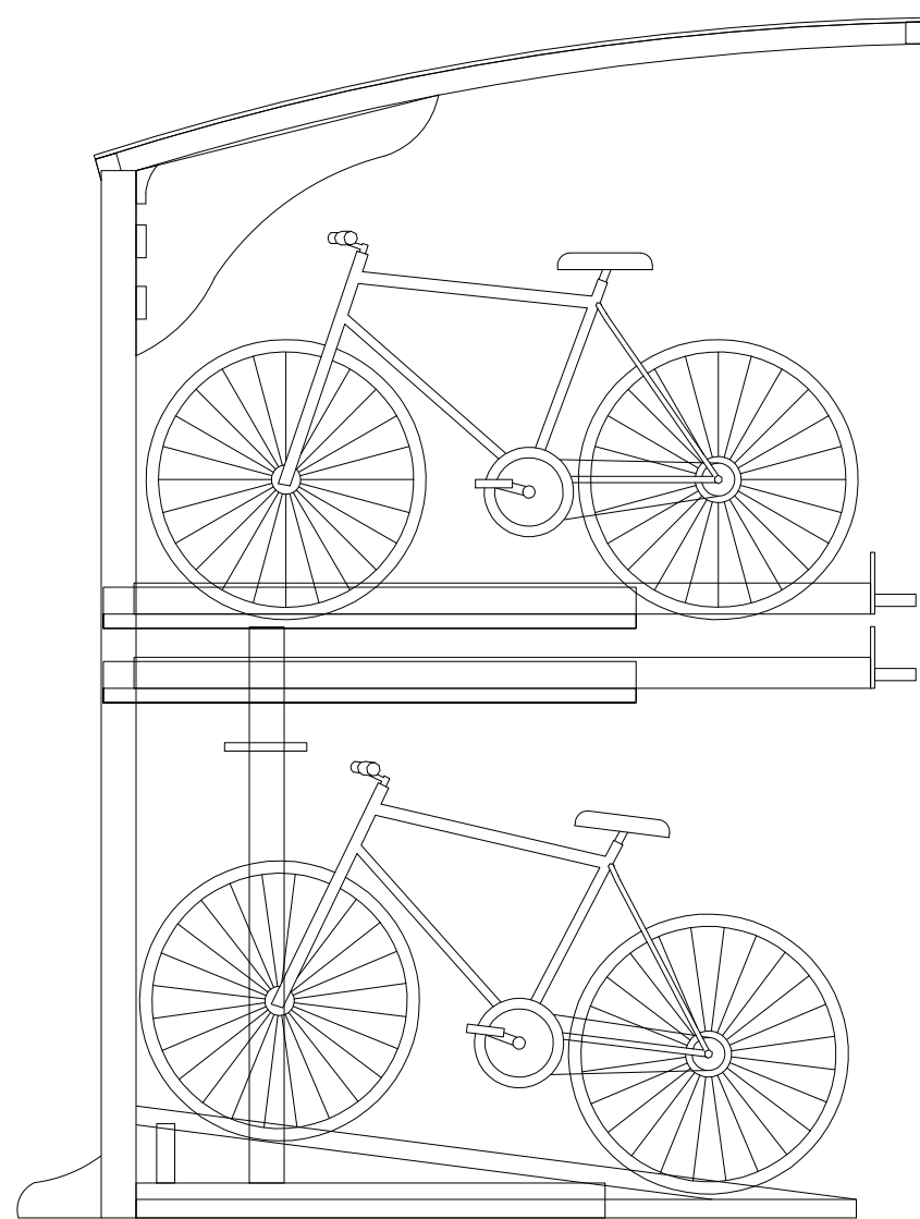
SIDE ELEVATION
