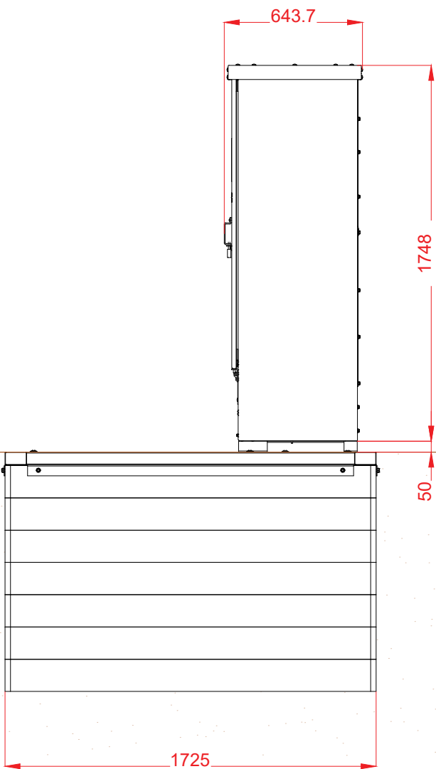
SIDE ELEVATION
