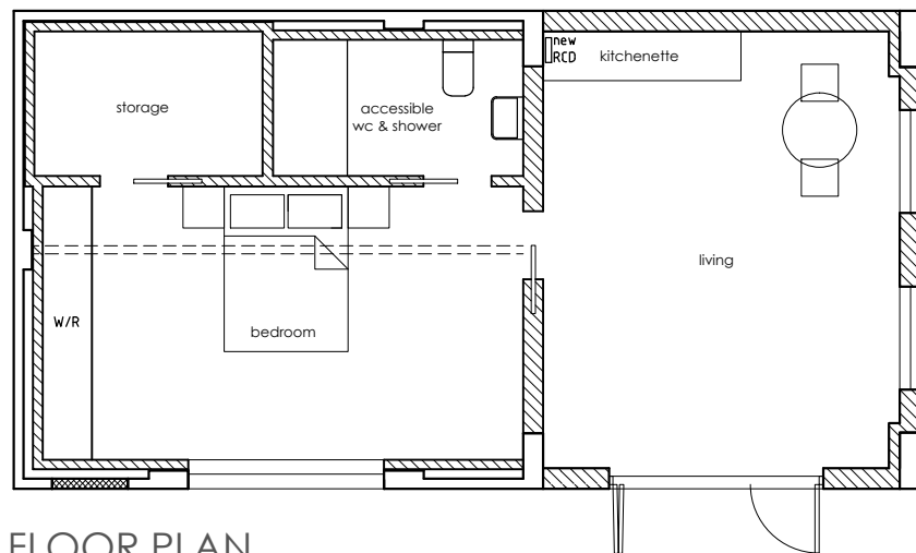
FLOOR PLAN
