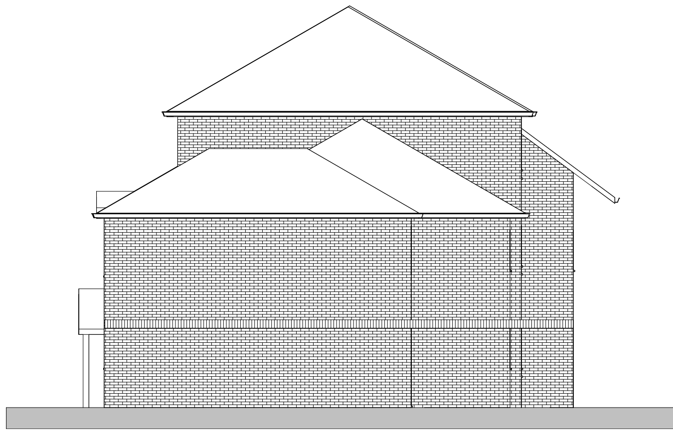
Proposed Side Elevation A 1 : 100
