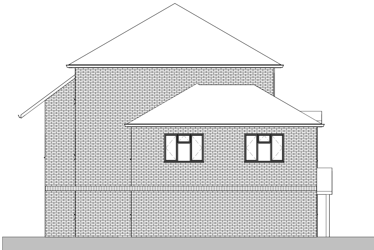
Proposed Side Elevation B 1 : 100
