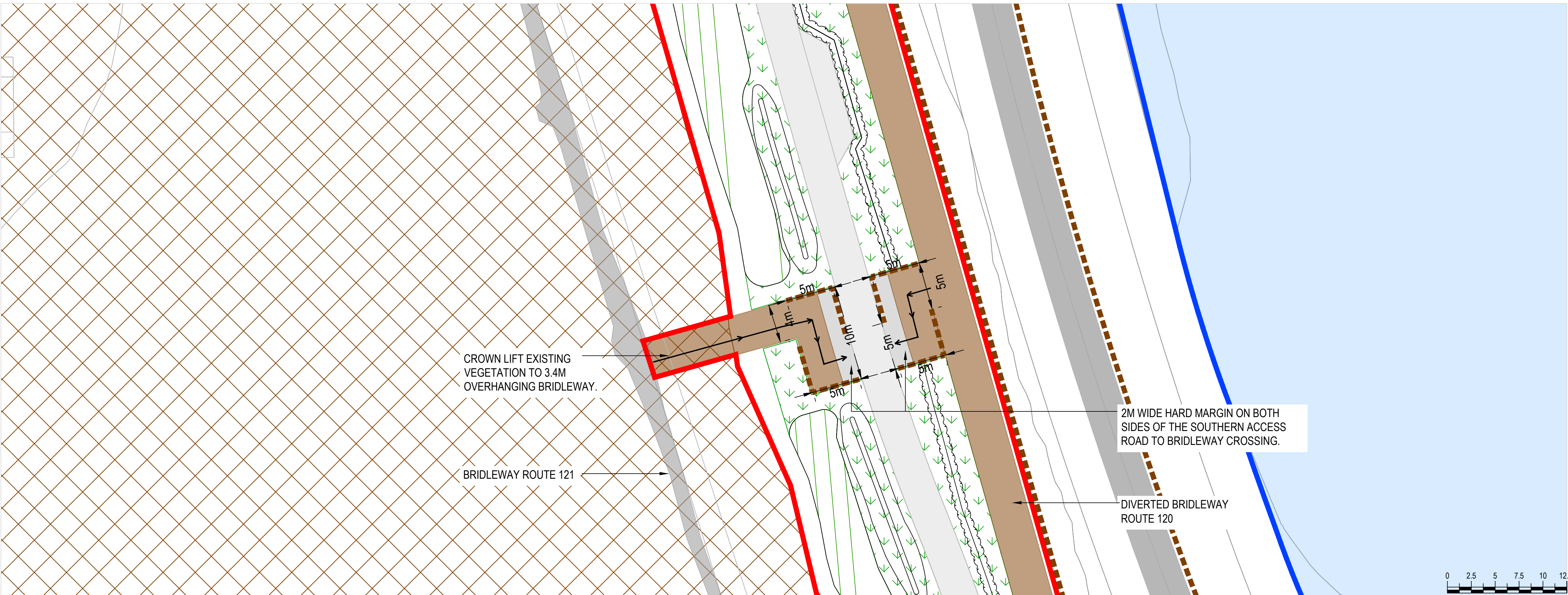
EQUESTRIAN CROSSING (PERMISSIVE) - FROM EXISTING BRIDLEWAY ROUTE 121 TO DIVERTED BRIDLEWAY ROUTE 120 / MAINTENANCE TRACK
