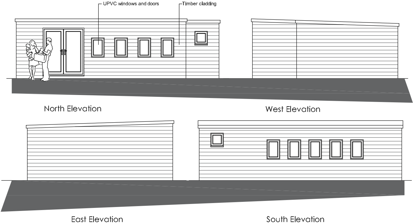
Proposed Elevations
