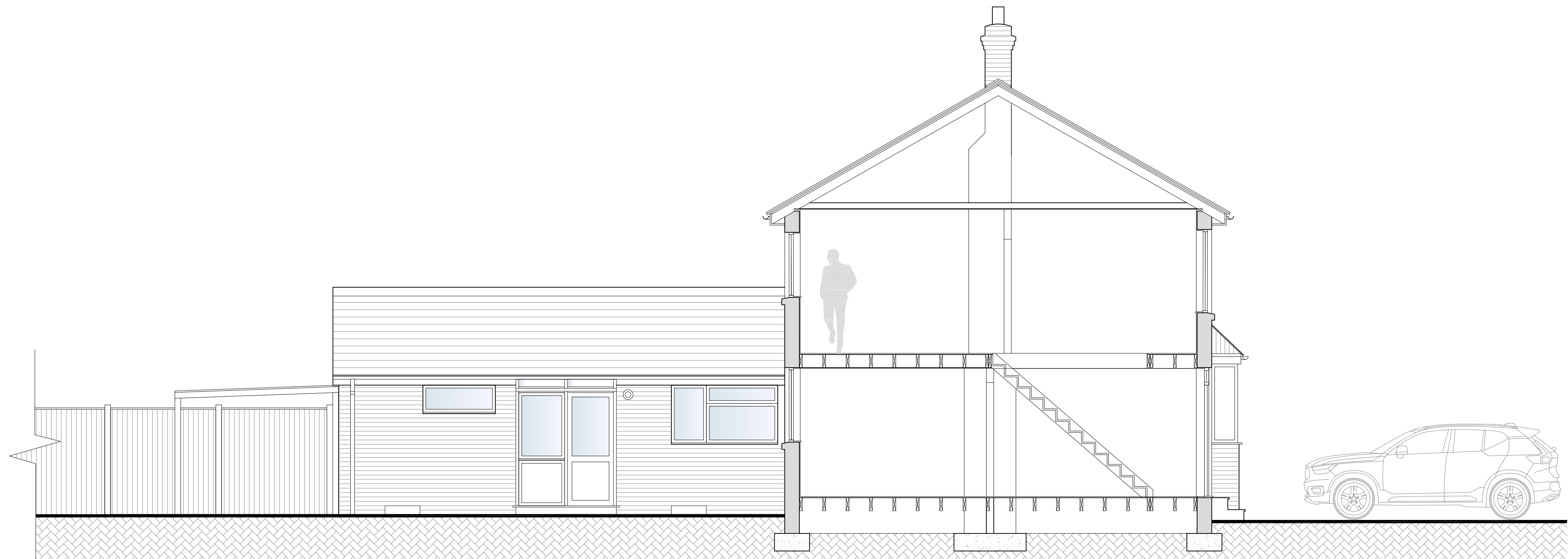
2 ELEVATION PART SECTION B-B G101 EXISTING SIDE ELEVATIONS SCALE @1:50
