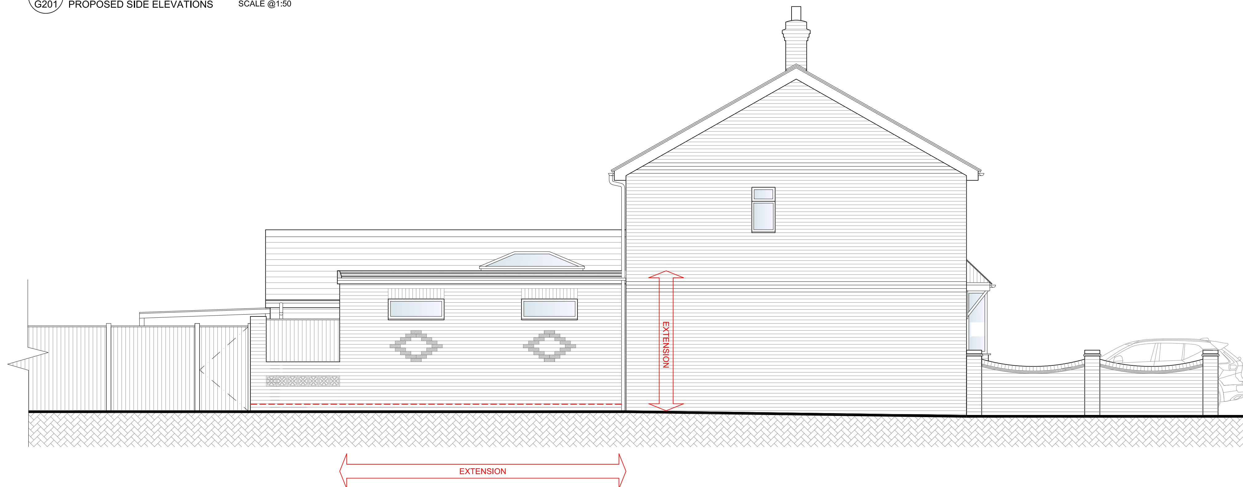
1 ELEVATION A--A G201 PROPOSED SIDE ELEVATIONS SCALE @1:50
