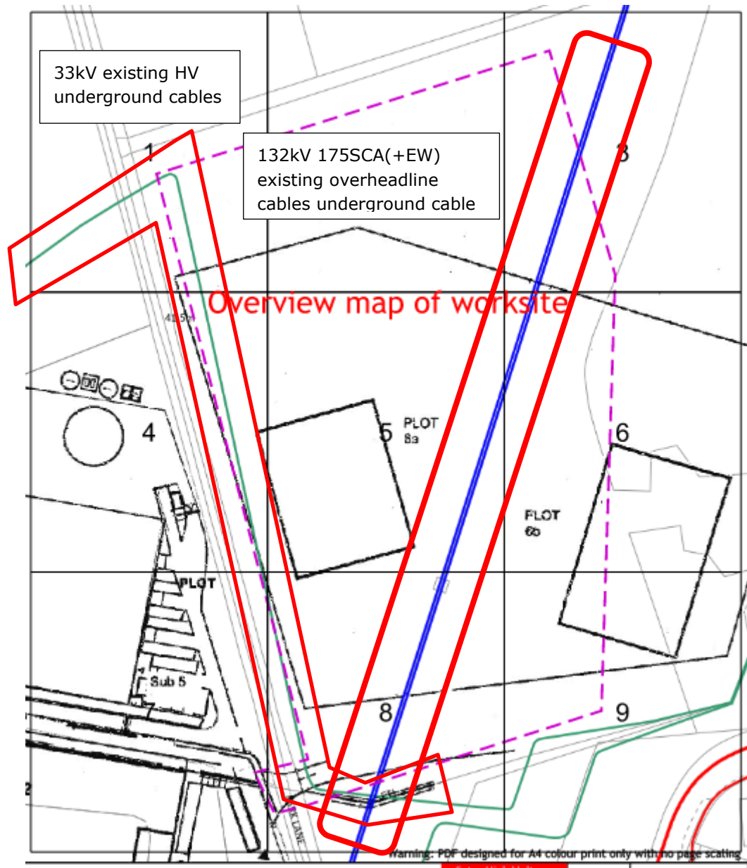
Figure 2 Existing HV SSEN network (Not To Scale)
