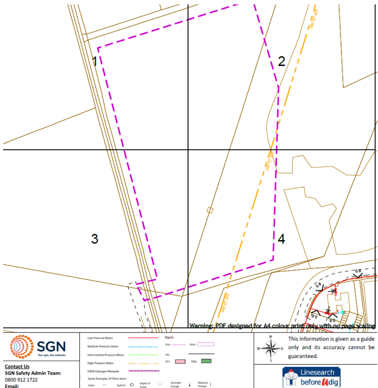
Figure 3: Existing Gas Network SGN at Plot 6 (not to scale) showing high pressure main
