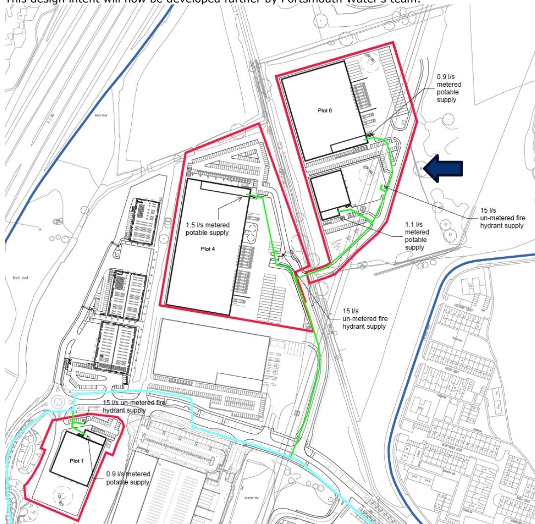
Figure 4: Proposed new water infrastructure (green denotes new services, light blue approx. existing water service location)
