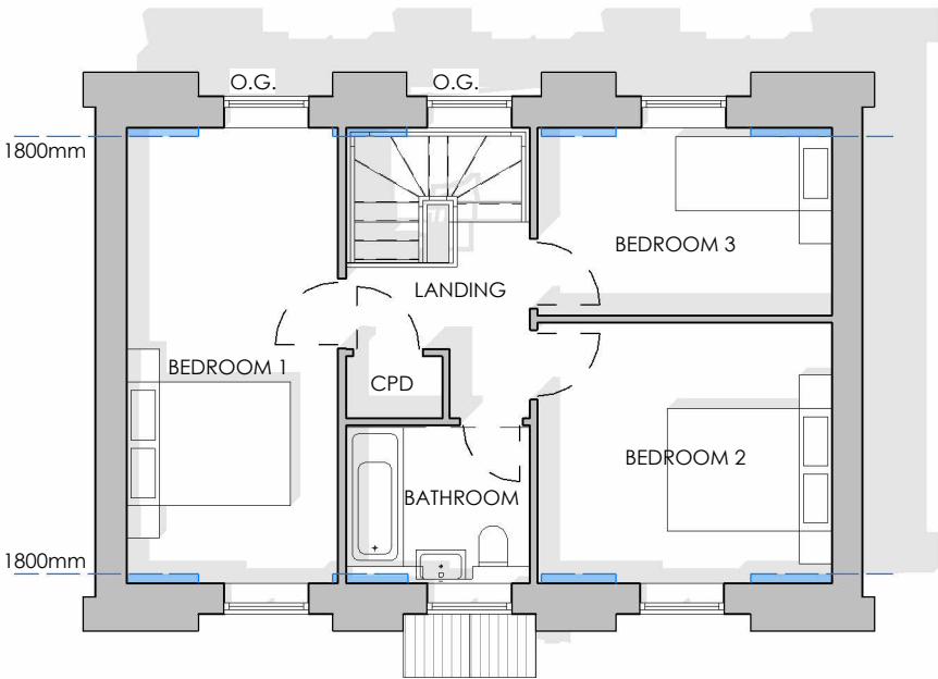
Proposed First Floor Plan 1 : 100
