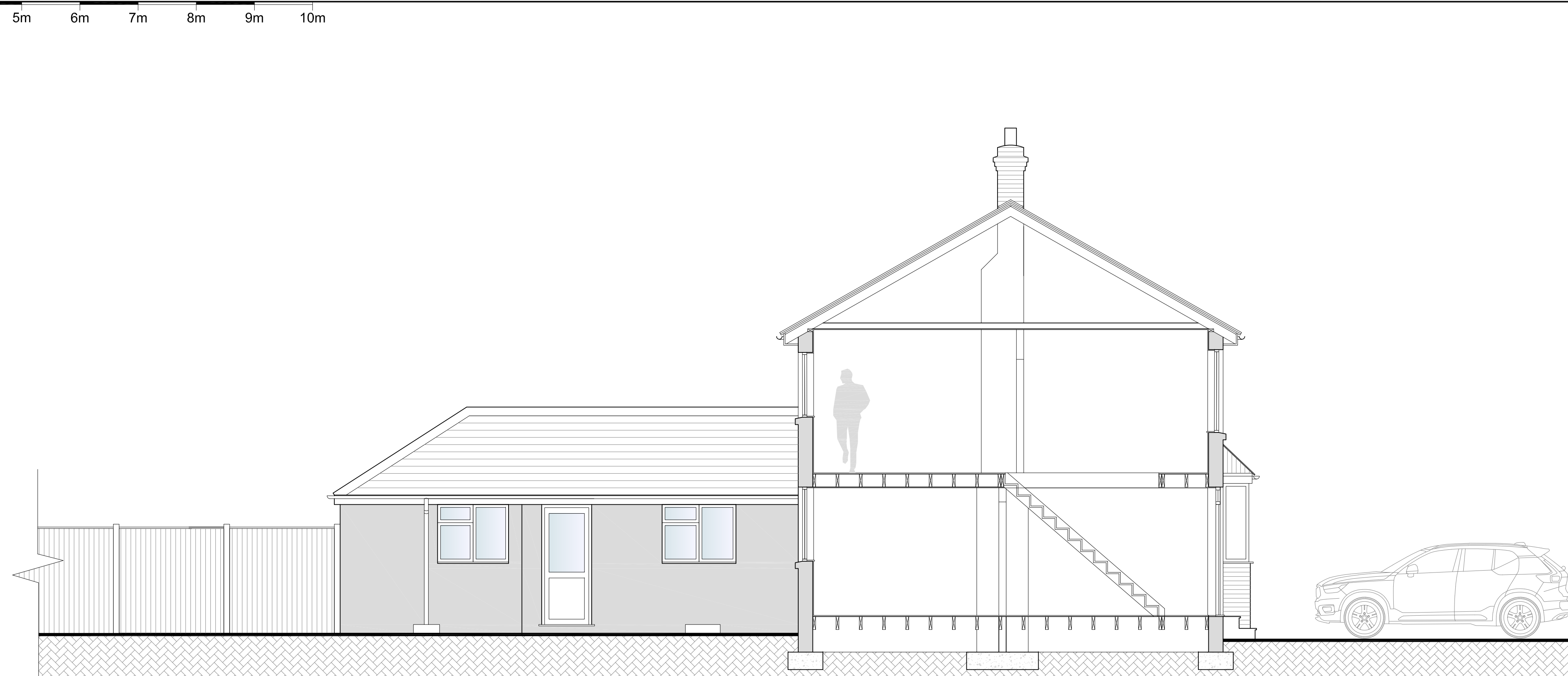
2 ELEVATION PART SECTION B-B G101 EXISTING SIDE ELEVATIONS SCALE @1:50
