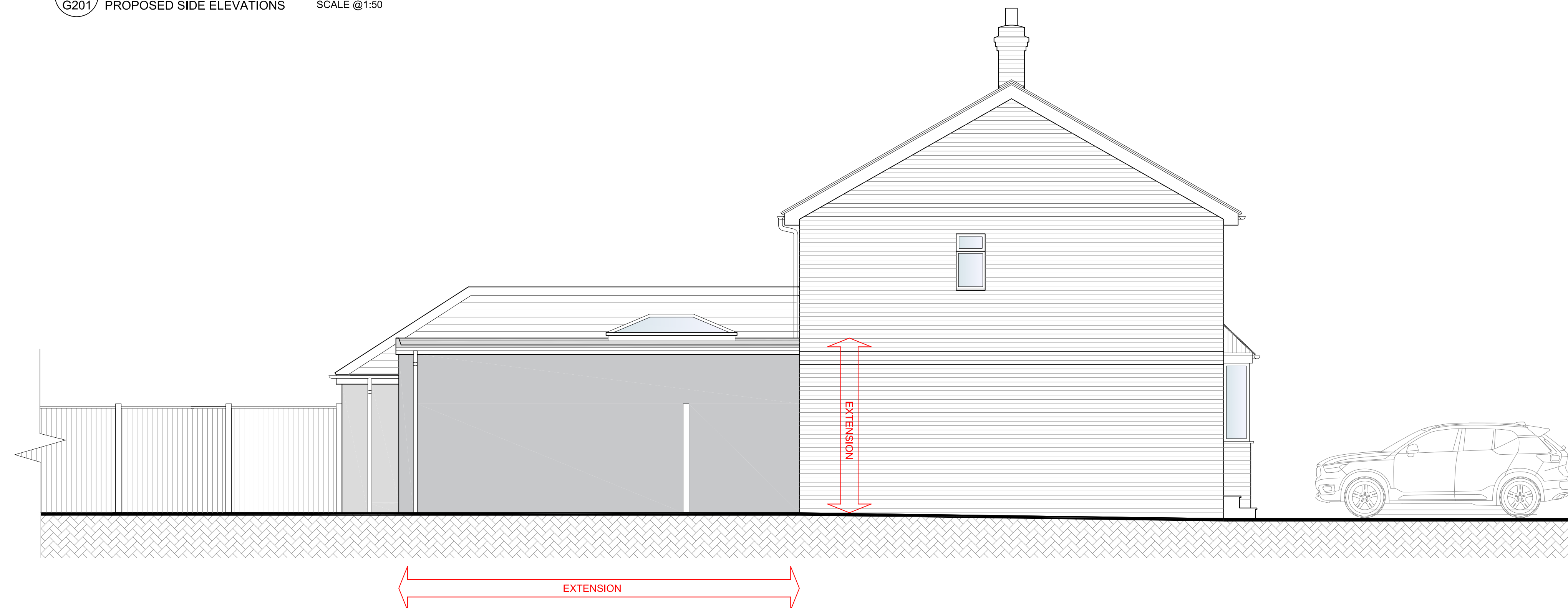
1 ELEVATION A--A G201 PROPOSED SIDE ELEVATIONS SCALE @1:50
