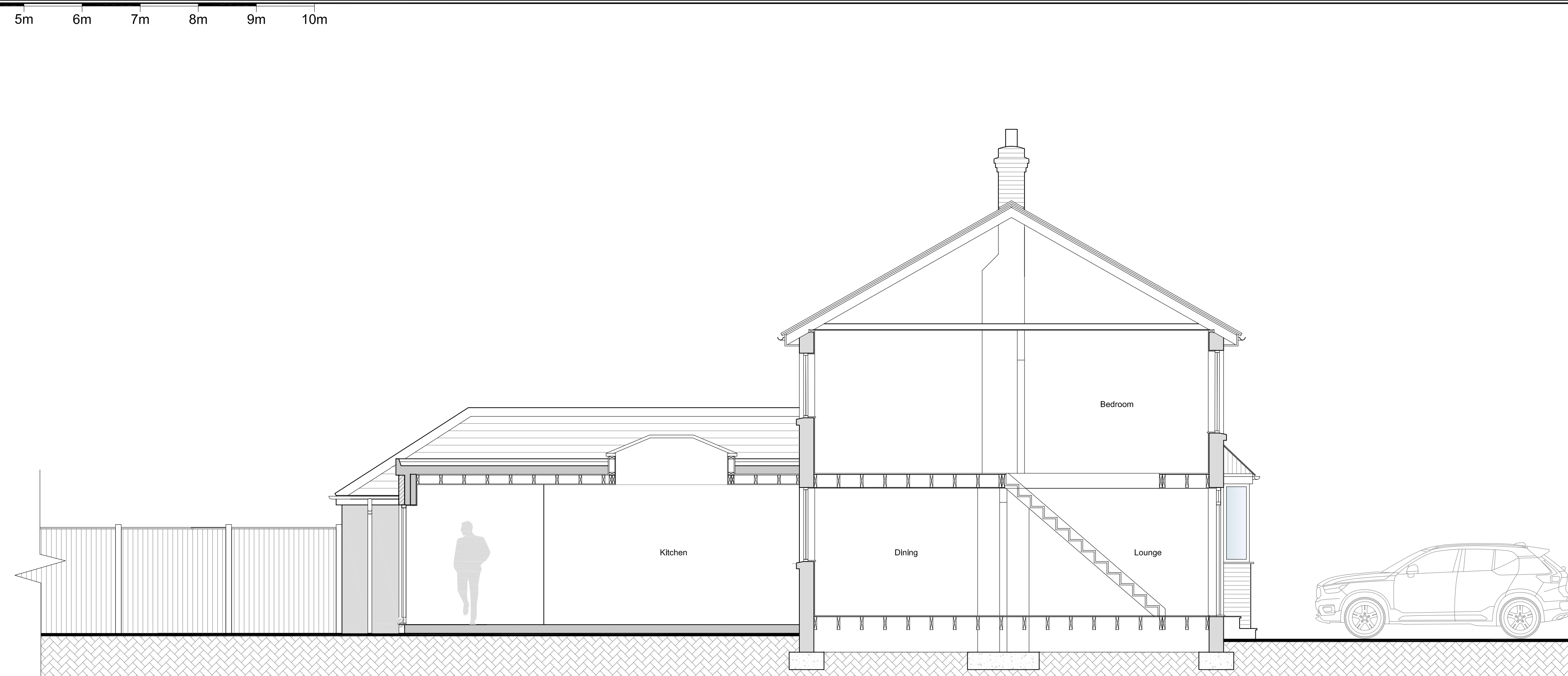
2 ELEVATION PART SECTION B-B G201 PROPOSED SIDE ELEVATIONS SCALE @1:50
