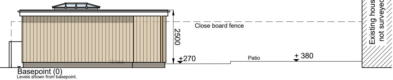
Site Section
