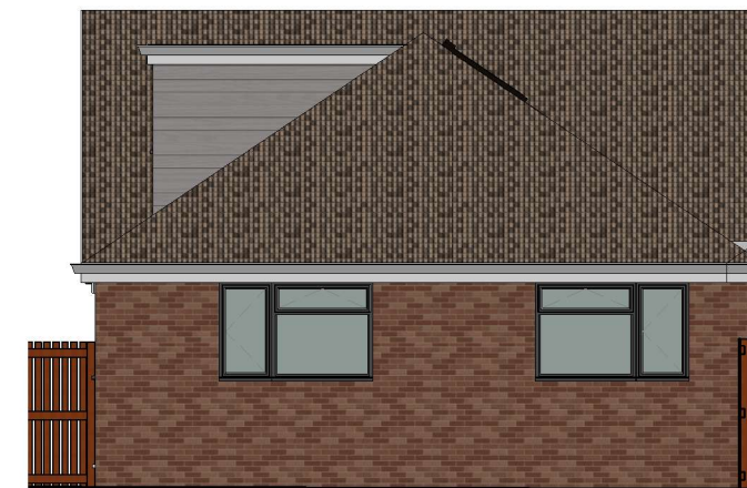
2 North Elevation 1 : 100
