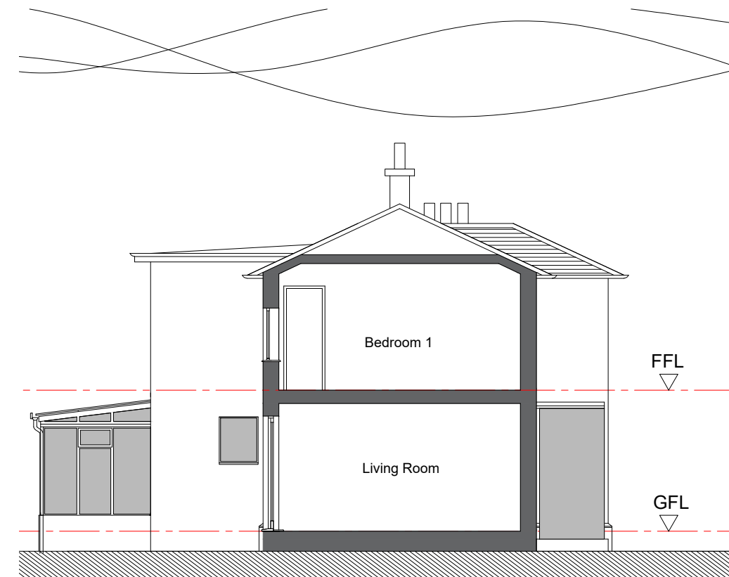
South Elevation
