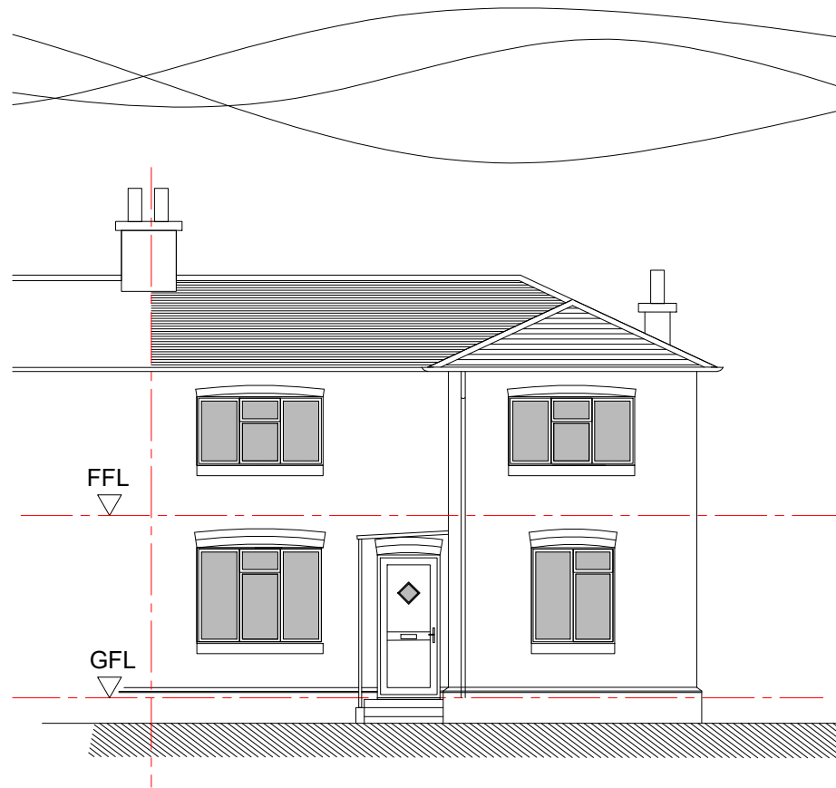
East Elevation
