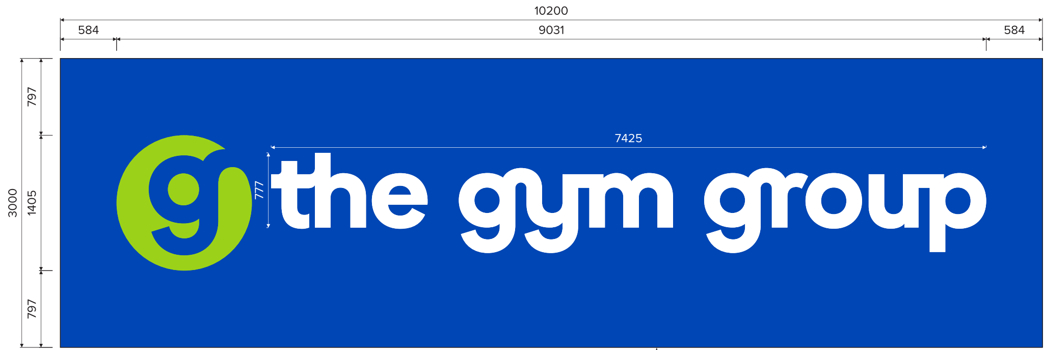
FACE VIEW @1:40
