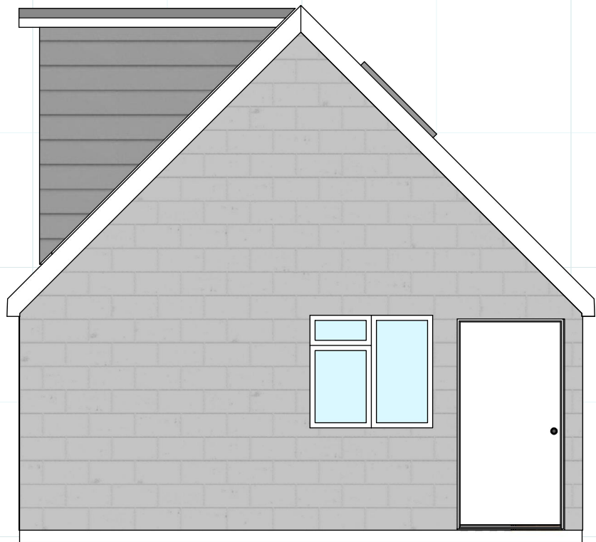
REAR ELEVATION
