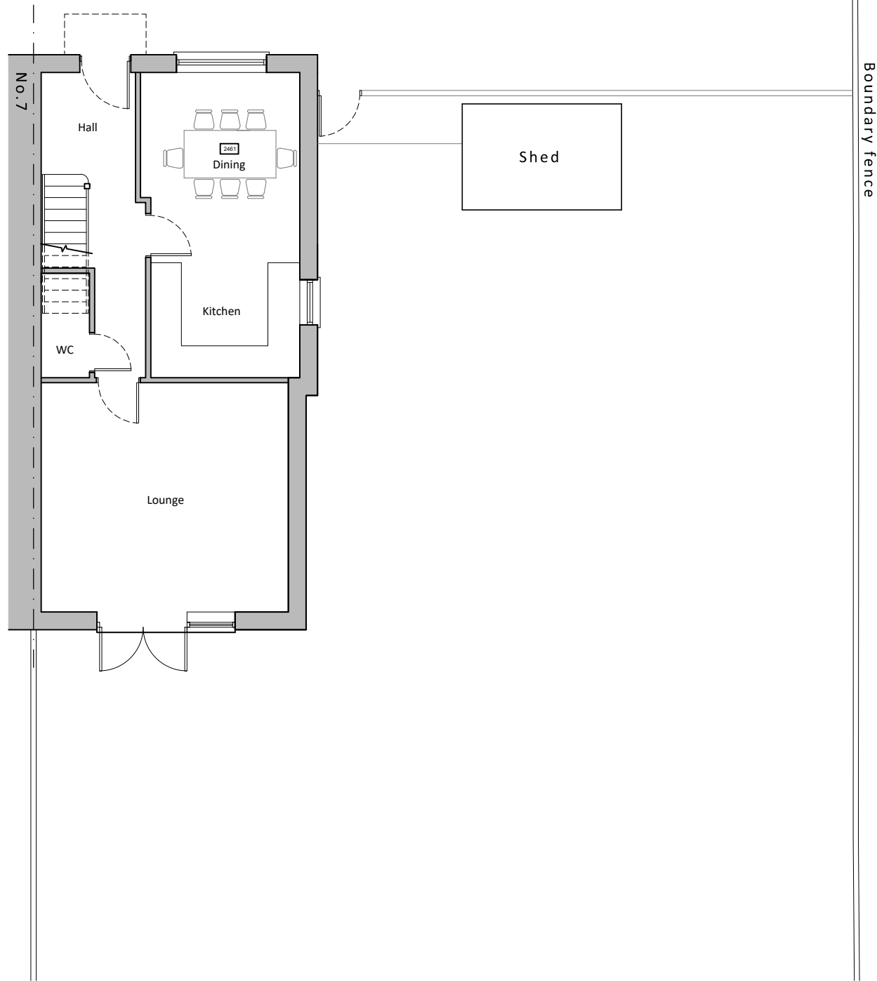
Ground floor
