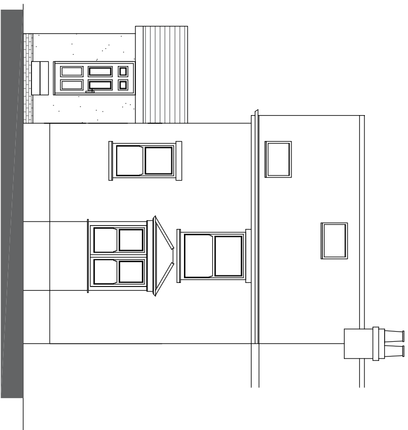
South Elevation
