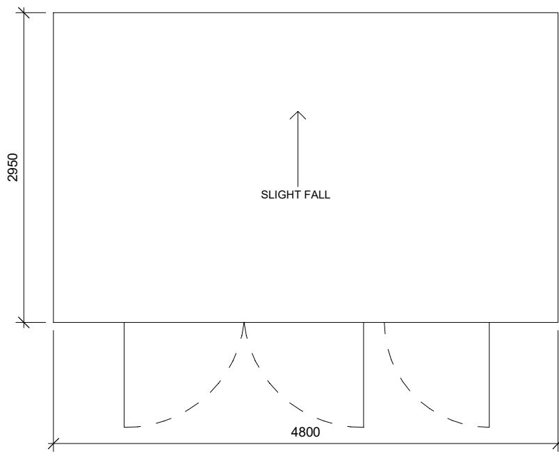
PROPOSED PLAN 1:50
