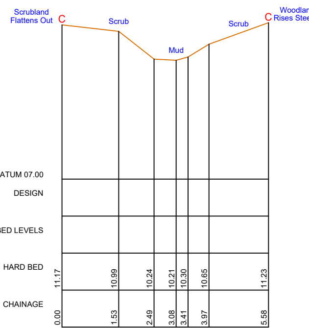
FIE01_1011 473628.28mE 106484.03mN Brg 154 Open Channel
