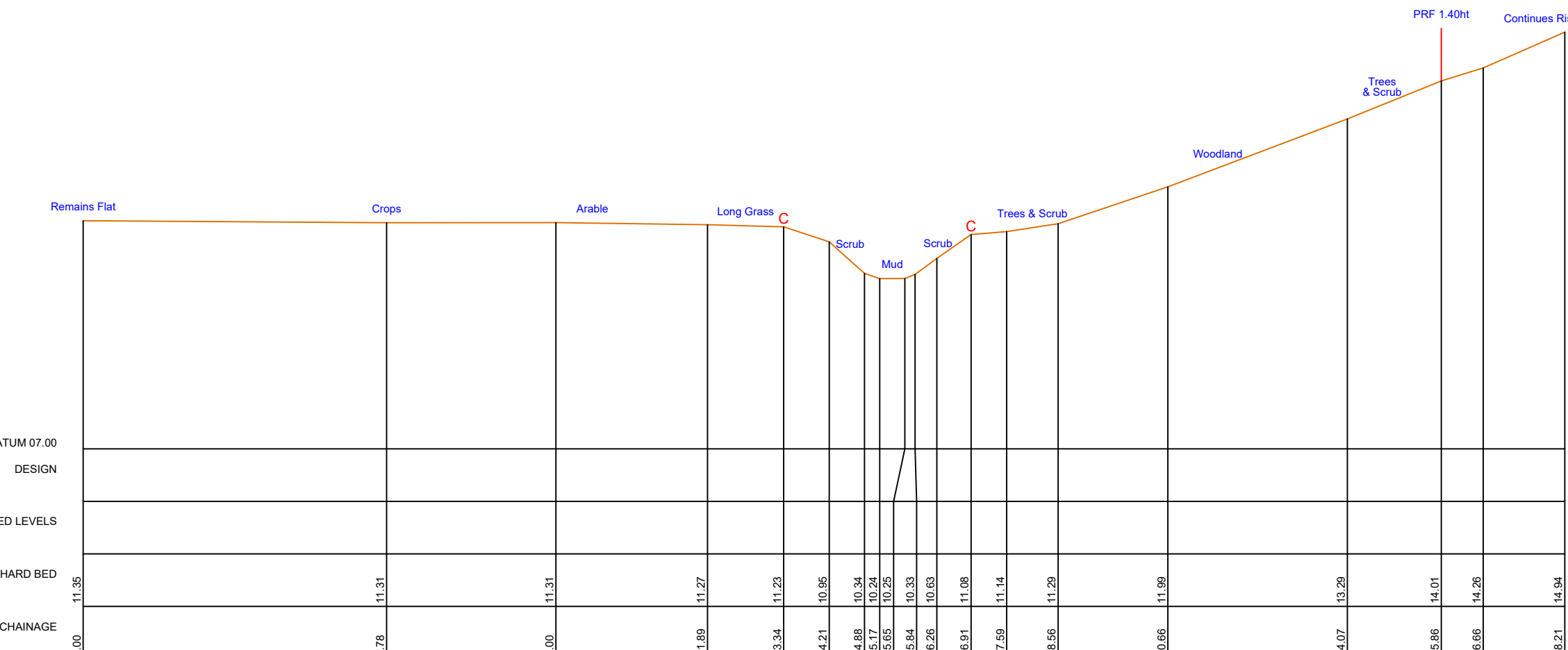
FIE01_0897 473733.78mE 106532.27mN Brg 163 Open Channel
