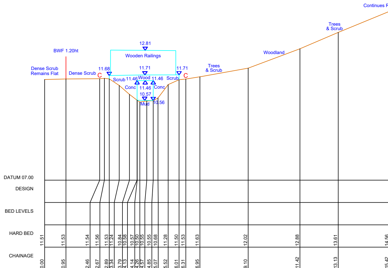
FIE01_1023 473617mE 106480.61mN Brg 158 Culvert Entrance Tunnel Length = 2.0m
