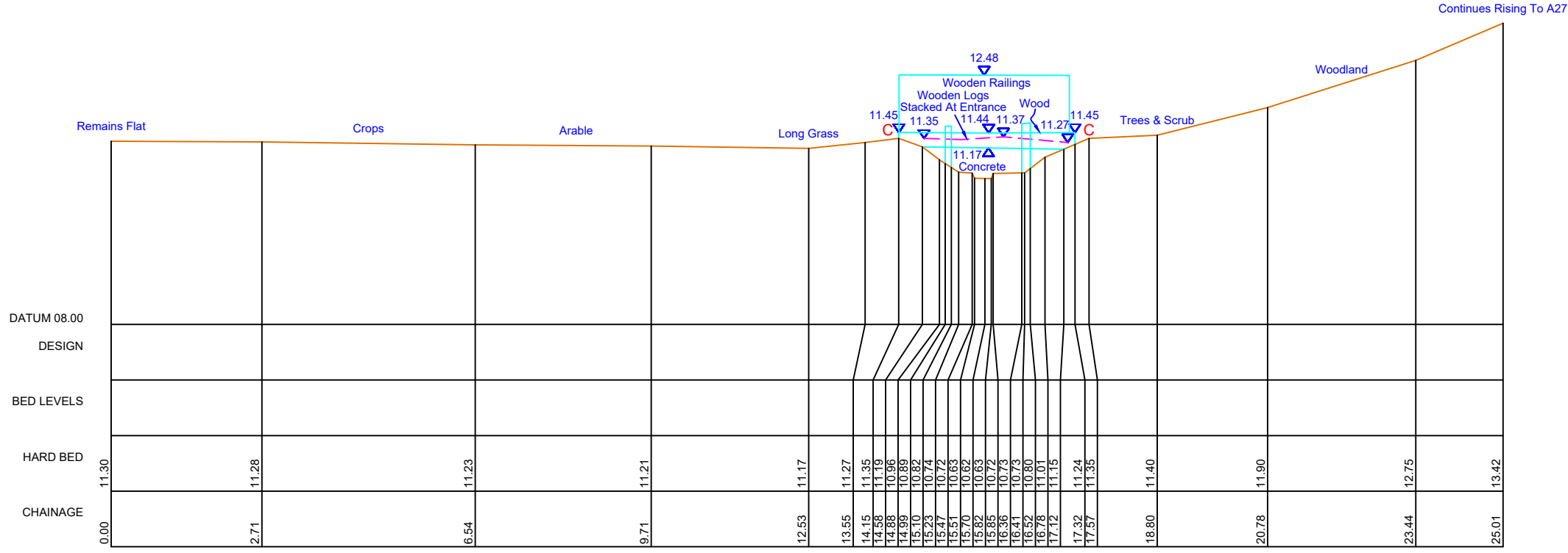
FIE01_0766 473865.65mE 106557.41mN Brg 176 Footbridge US Face Tunnel Length = 2.0m
