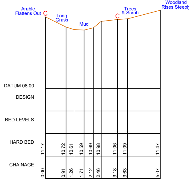
FIE01_0769 473863.22mE 106542.92mN Brg 170 Open Channel
