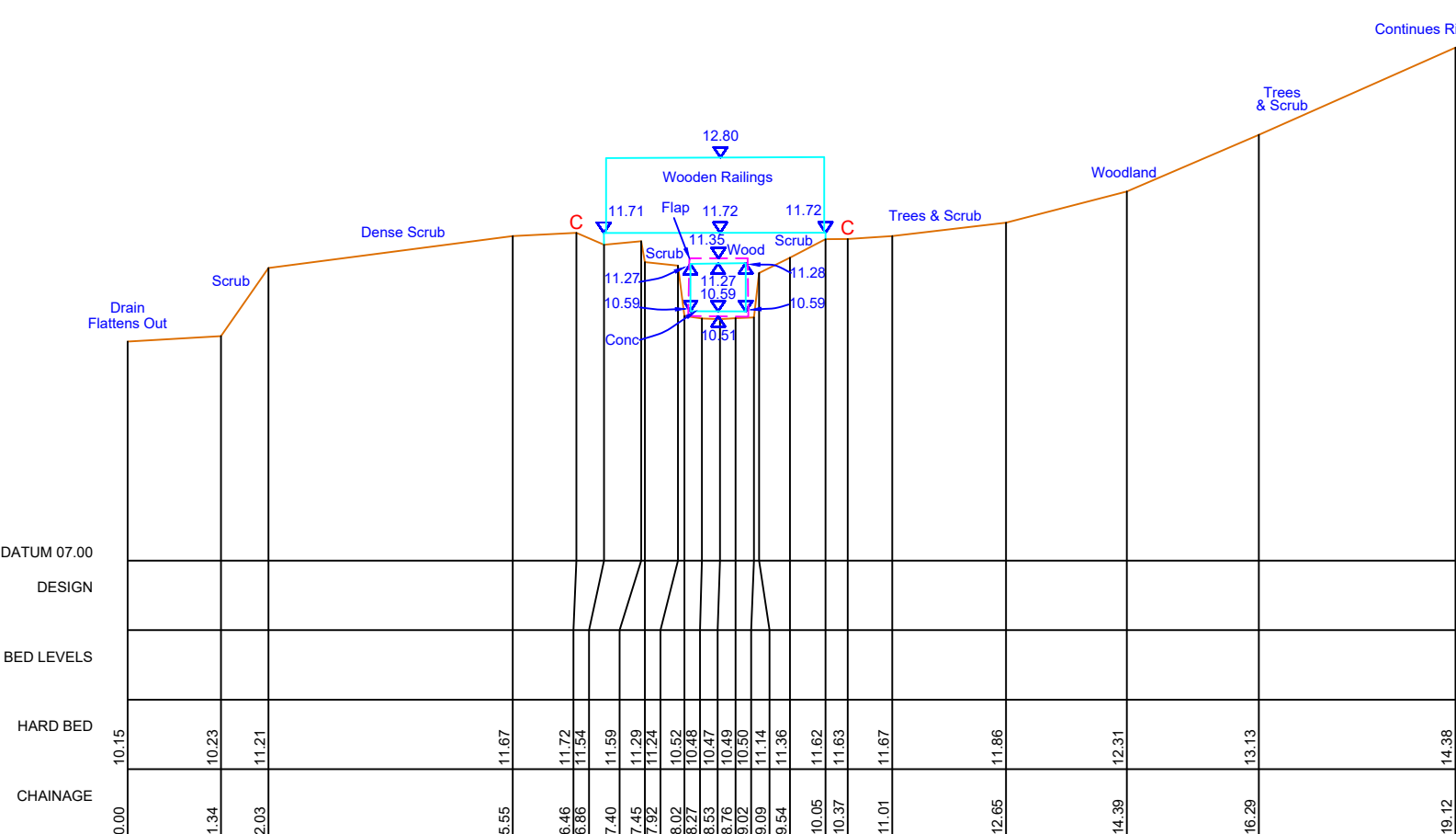
FIE01_1021 473617.48mE 106485.17mN Brg 159 Culvert Exit Tunnel Length = 2.0m
