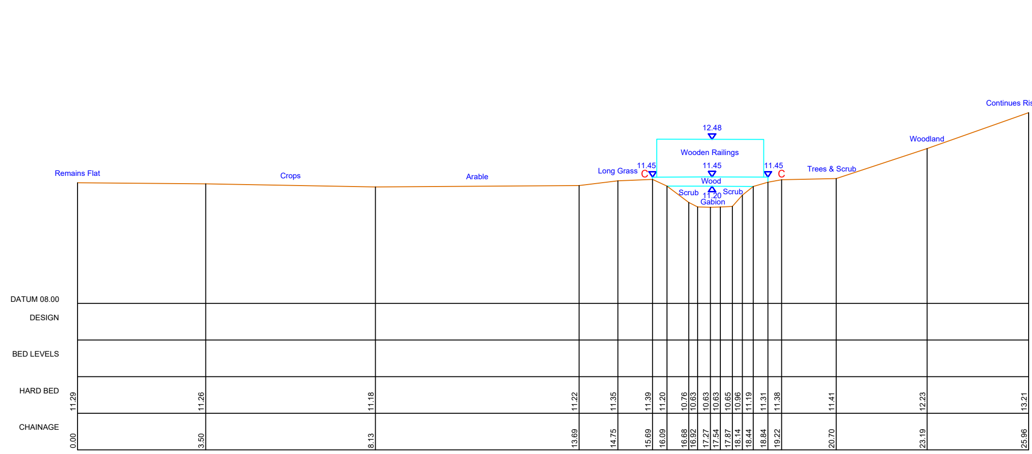
FIE01_0764 473867.82mE 106559.17mN Brg 175 Footbridge DS Face Tunnel Length = 2.0m
