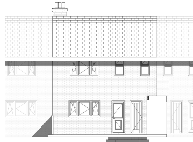
Proposed Elevation-Rear
