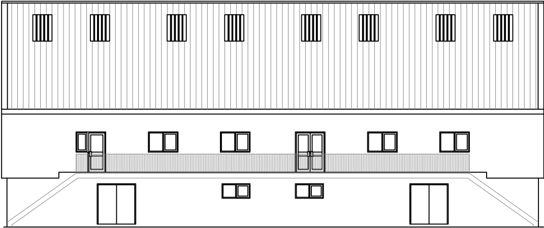
North Elevation 1:200
