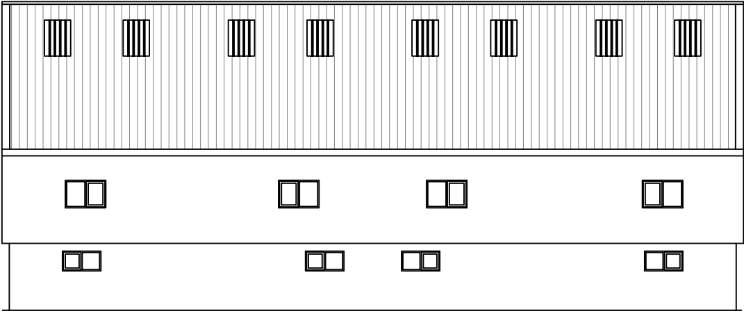
South Elevation 1:200
