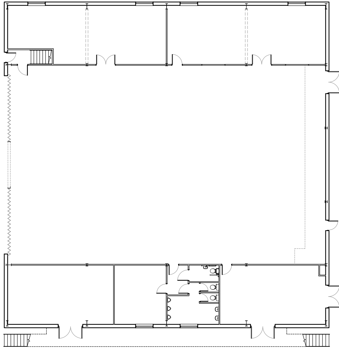
Ground Floor 1:200
