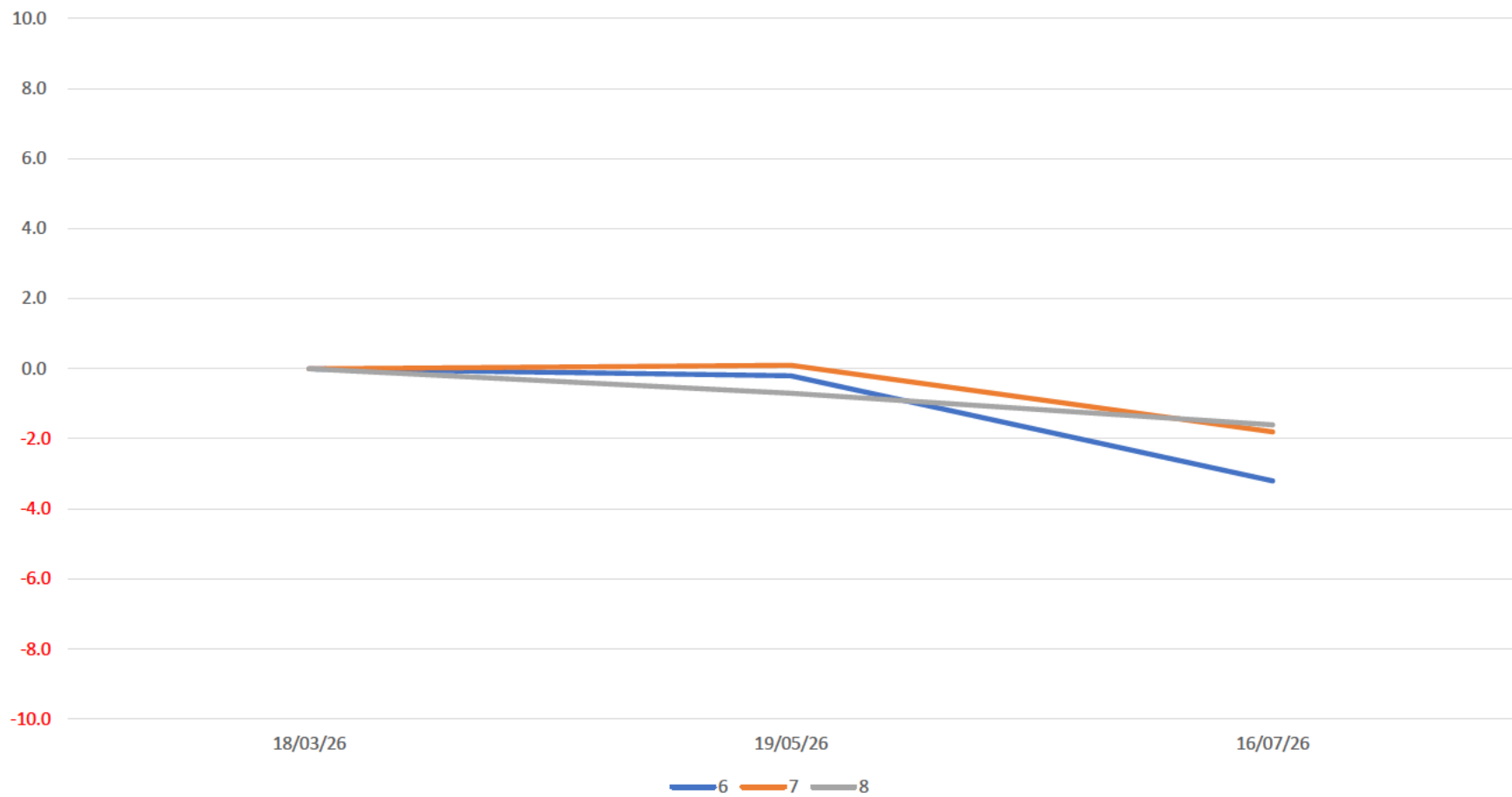
Relative Movements in mm
