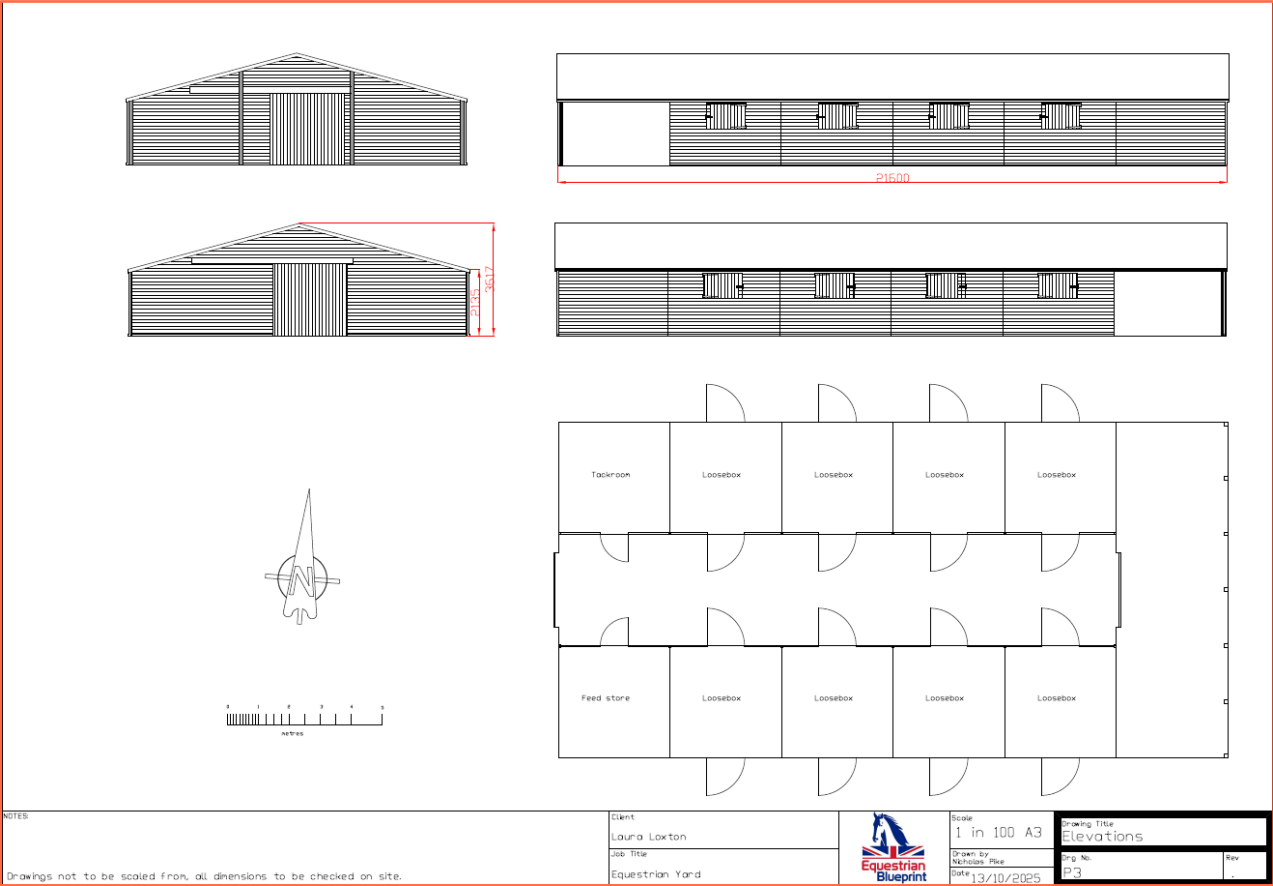
Figure 6: Floor plan and elevations (Source: Equestrian Blueprint)
