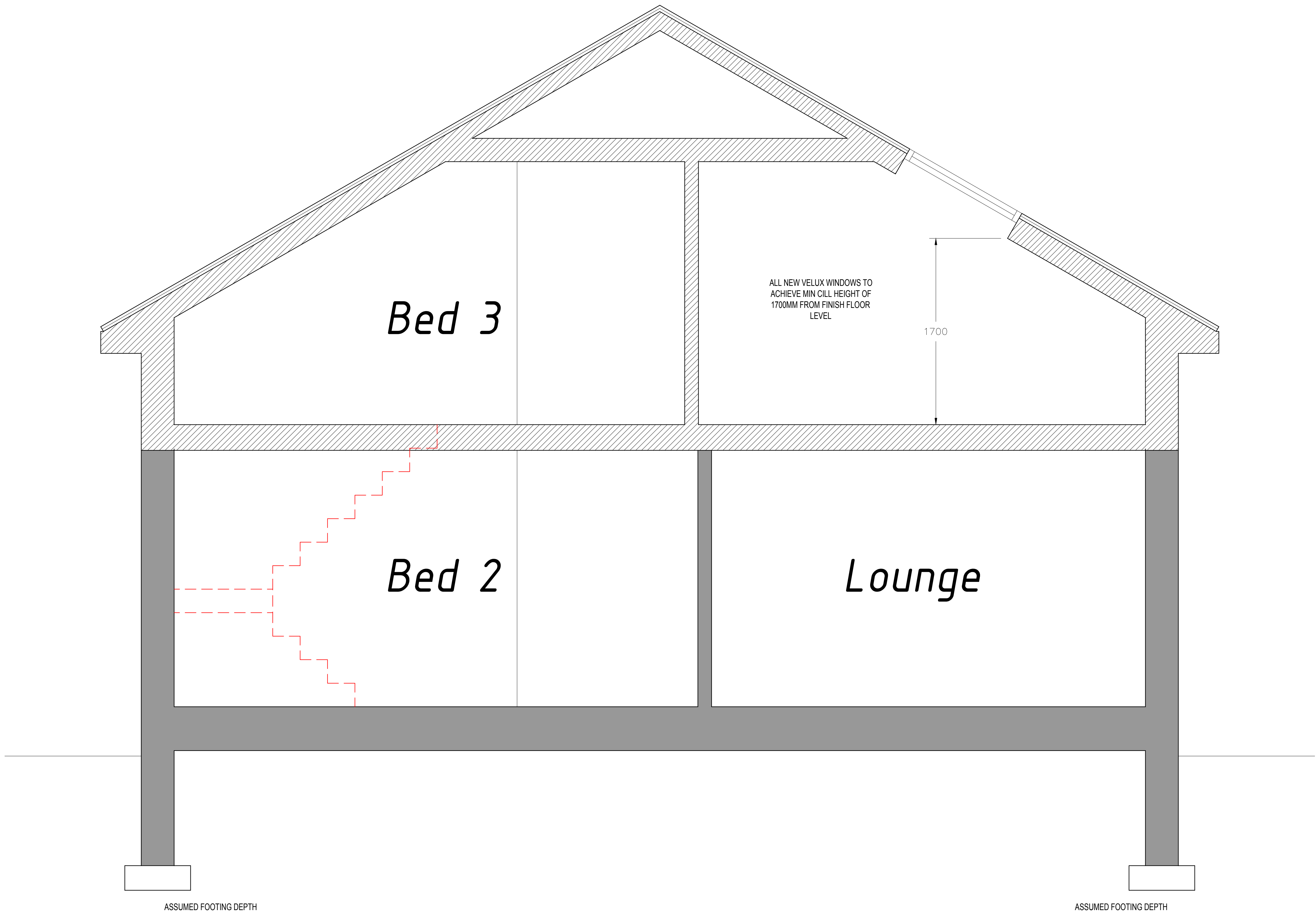
PROPOSED SECTION SCALE 1: 20@A1
