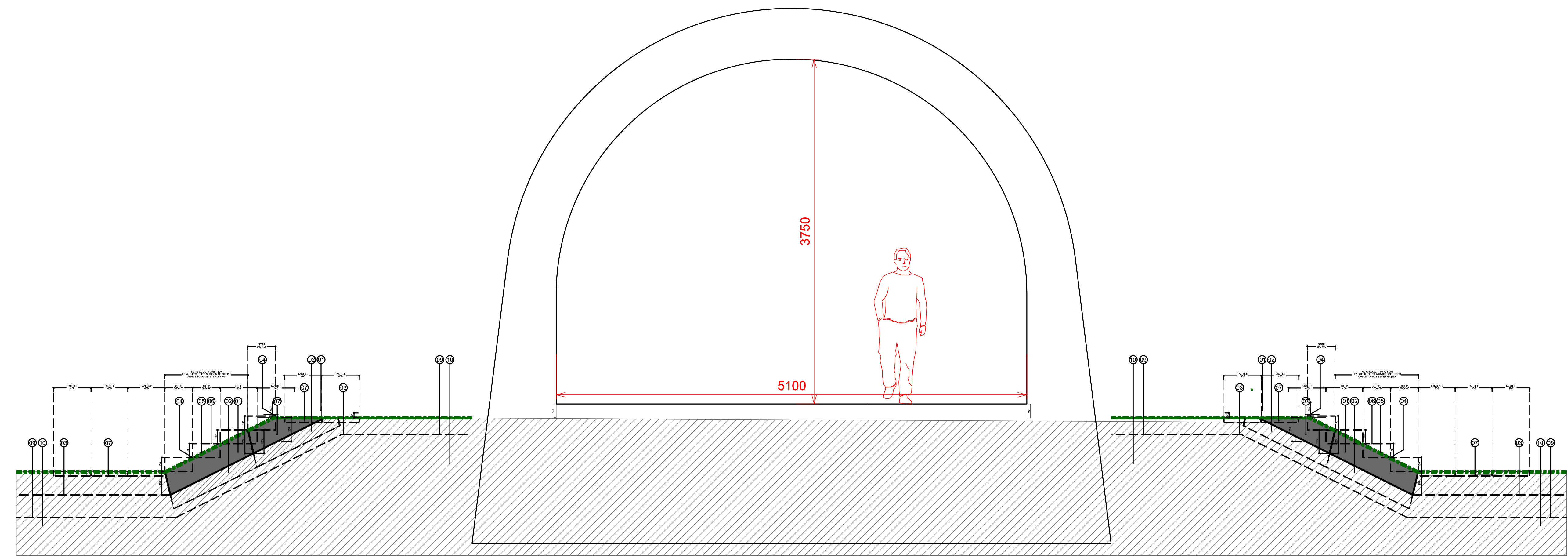
02 STEPS - FLANK KERB EDGING - SECTION SCALE 1:10 @ A1
