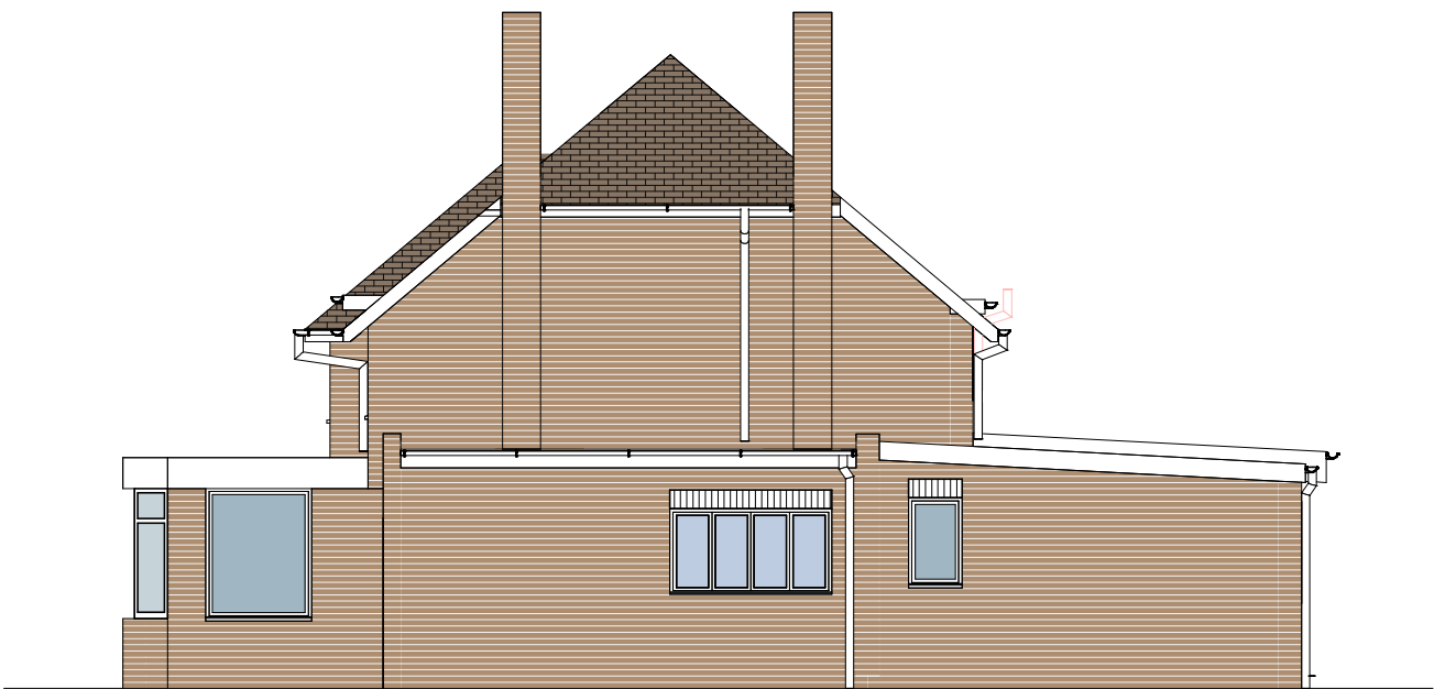
Proposed Side Elevation (South) 1 : 100
