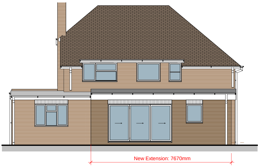
Proposed Rear Elevation (East) 1 : 100
