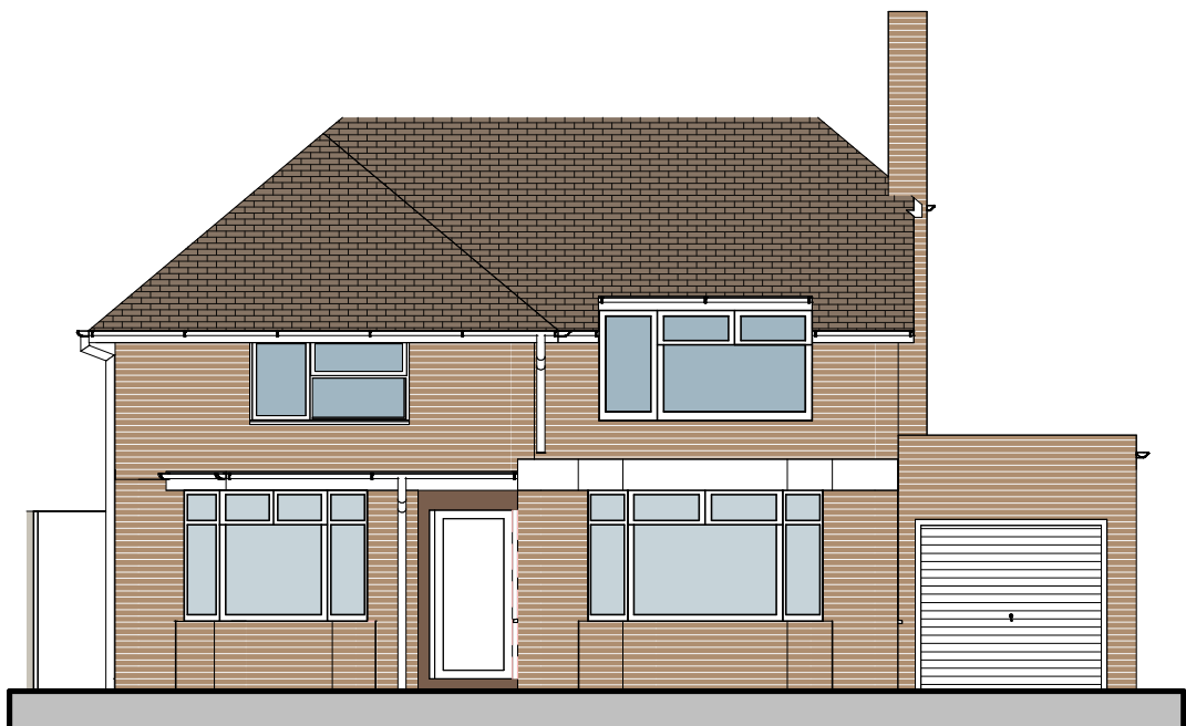
Proposed Front Elevation (West) 1 : 100
