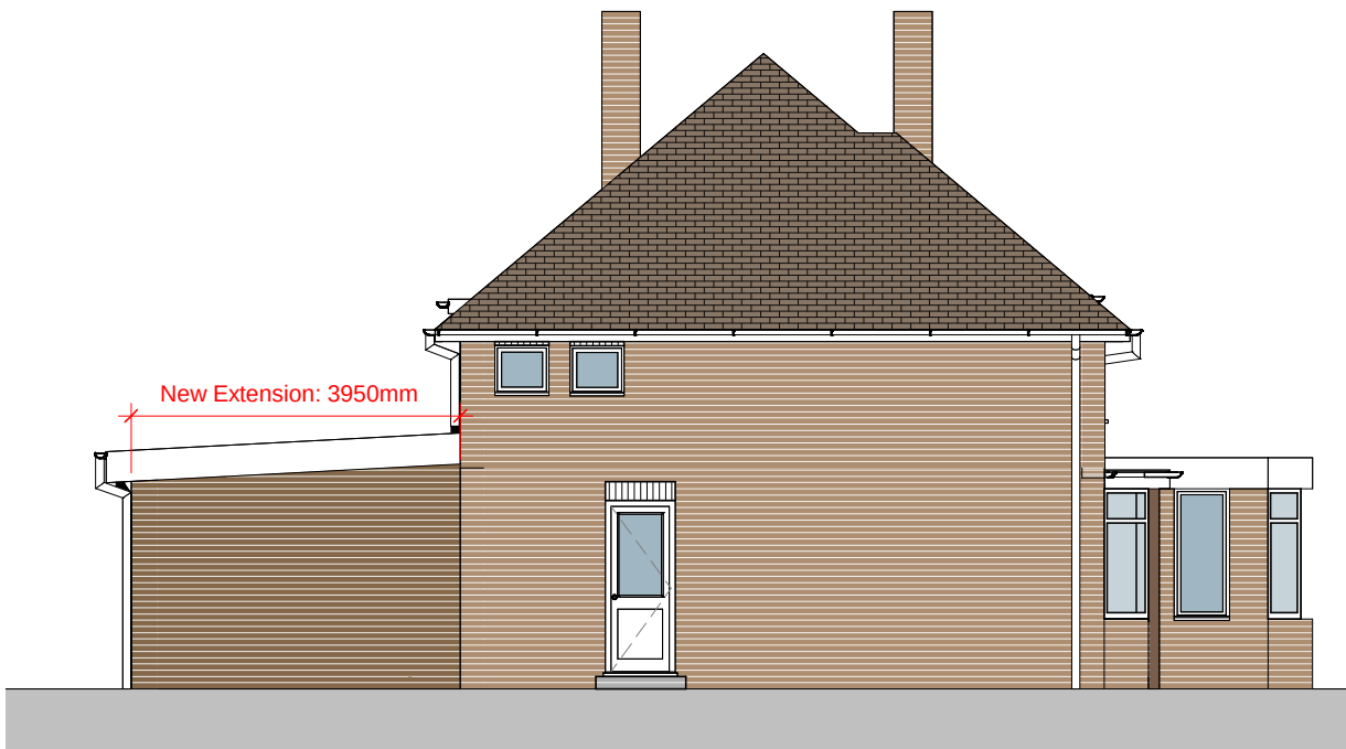
Proposed Side Elevation (North) 1 : 100
