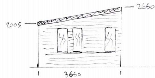
SIDE ELEVATION
