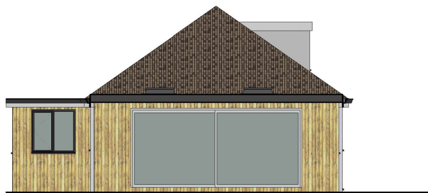
3 South Elevation
