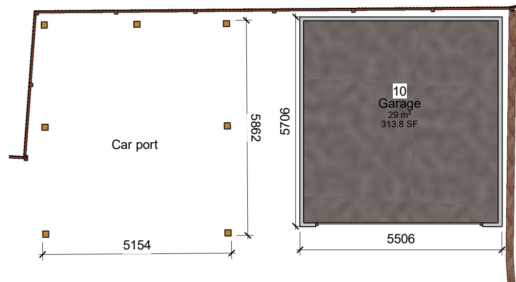
5 Garage Car Port Plan 1 : 100
