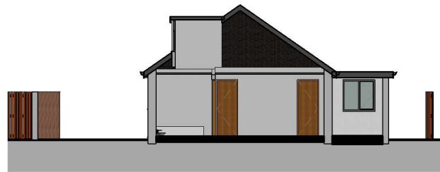
2 East West Site Section 1 : 200
