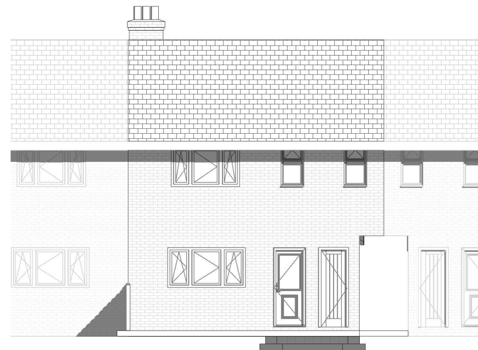
Proposed Elevation-Rear
